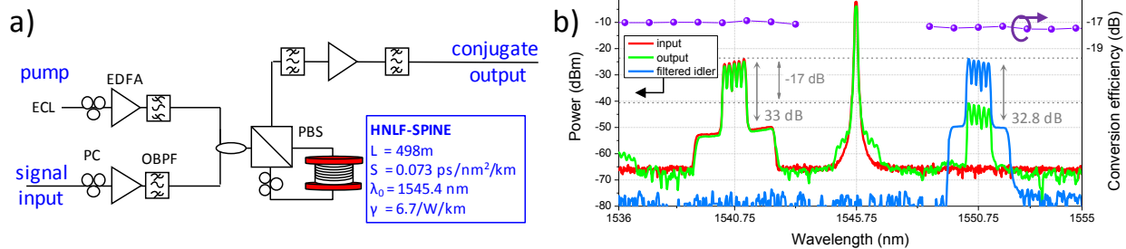
Fig. 2. (a) Setup of polarization-diversity based OPC module and (b) OPC input and output spectra, and CE of the HNLF-SPINE.
