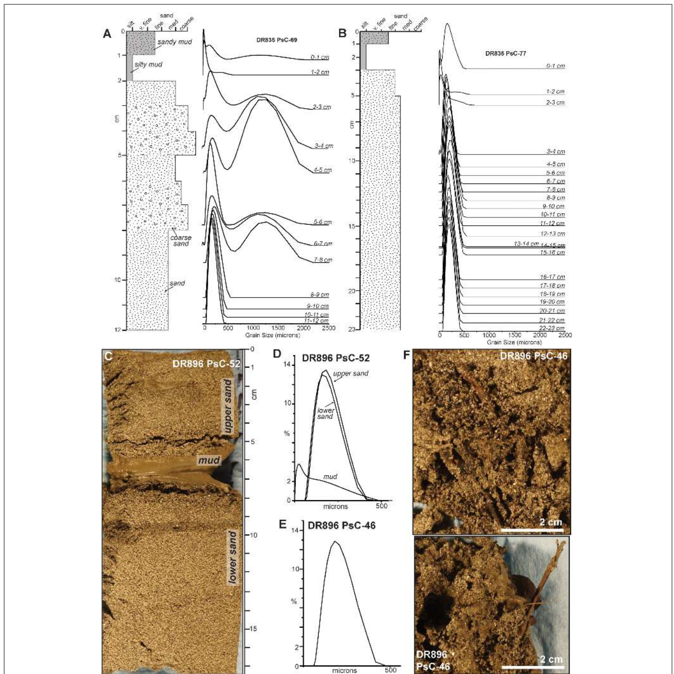
FIGURE 8 | Remotely operated vehicle (ROV) pushcore samples acquired near MS7. (A,B) Pushcores acquired in April 2016, following the January 15, 2016 event, shown as schematic log ( left ) and grain-size distributions ( right ). Stratigraphy and coarse grain size populations differ between these two closely spaced pushcores (57 m apart). See Figure 1B for sample locations. (C–F) Pushcores acquired in October 2016, after the September 1, 2016 event, shown as photographs and grain-size distributions. Woody plant material in sand is highlighted in (F) . See Figure 1C for sample locations.
