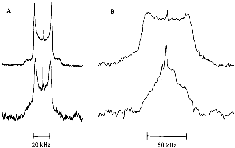
Fig. 11. ^2\text{H} -nmr spectra (at 46.1 MHz) of reconstituted functional sarcoplasmic reticulum. The natural lipids are exchanged to the extent of 99% with 1,2-di-elaidoyl- sn -glycerol-3-phosphocholine (DEPC). At least 90% of the DEPC is deuterated in both chains at the 9, 10 position, i.e. at the trans -double bond. The phase transition of DEPC occurs at about 10 °C.
