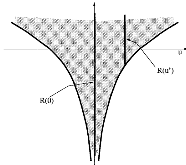
Figure 2. A locally sub-Lipschitz mapping continuous.
