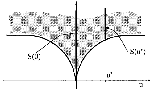
Figure 1. A mapping that isn't locally sub-Lipschitz continuous.
