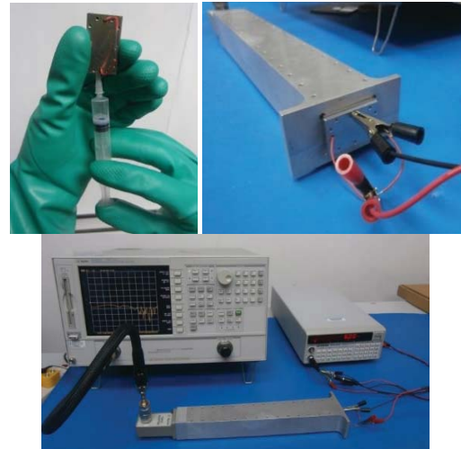
Fig. 5 LC filling in cavity, unit cell inserted in waveguide simulator and complete measurement set-up for scattering parameter measurements
