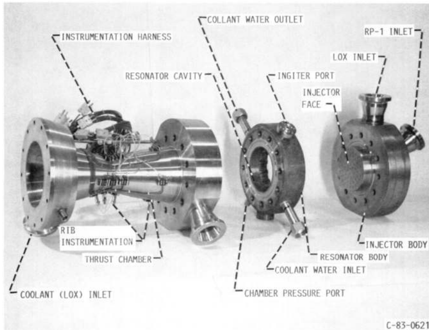
FIGURE 6.- THRUST CHAMBER, RESONATOR, AND INJECTOR.
