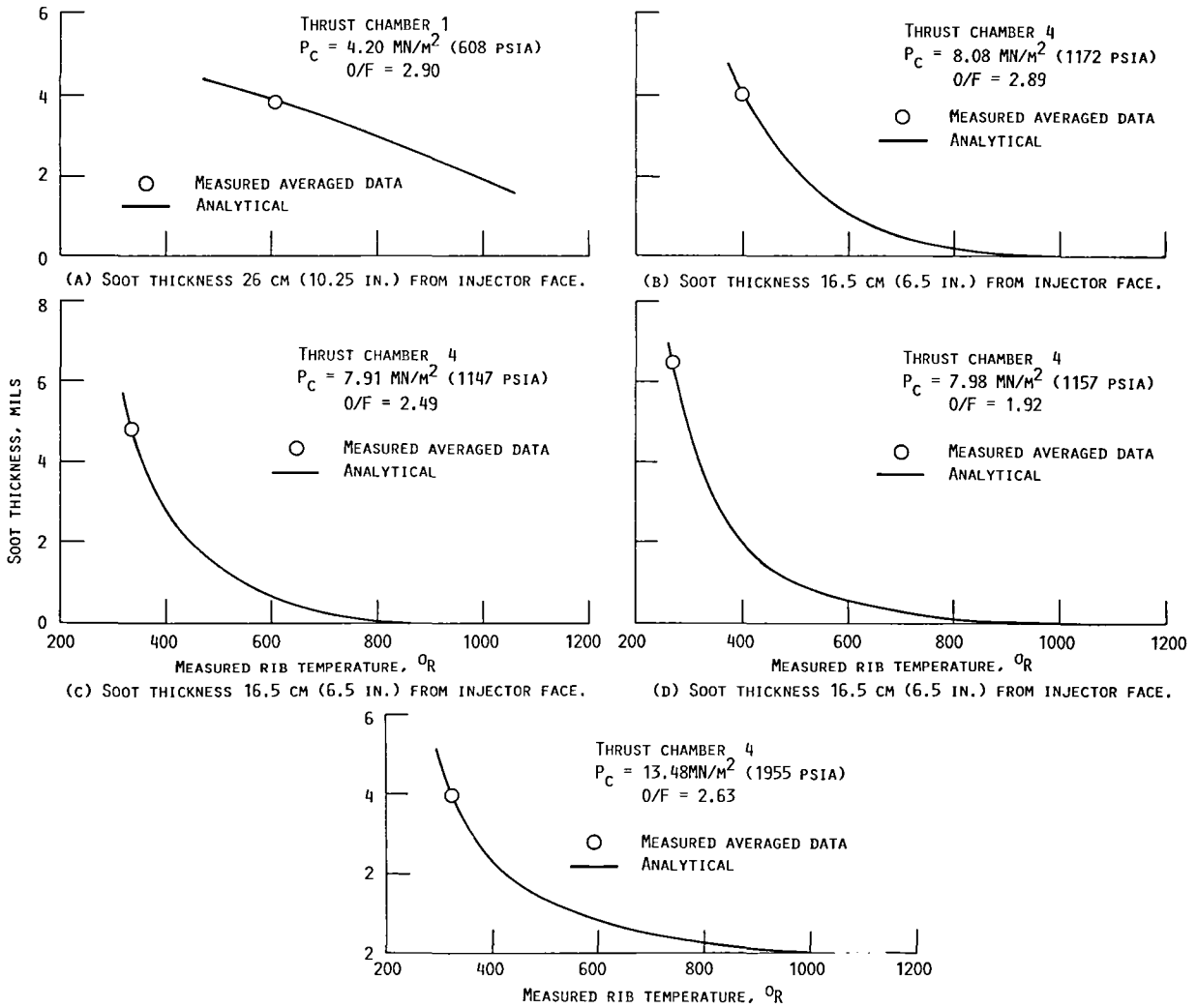
(E) SOOT THICKNESS 16.5 CM (6.5 IN.) FROM INJECTOR FACE. FIGURE 9.- SOOT THICKNESS DISTRIBUTION FOR CYLINDRICAL SECTION.
