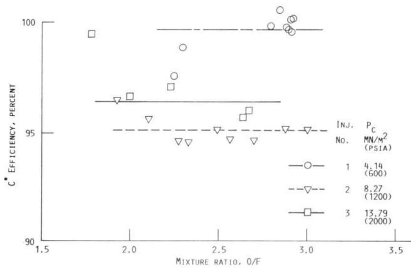
FIGURE 8.- INJECTOR PERFORMANCE.
