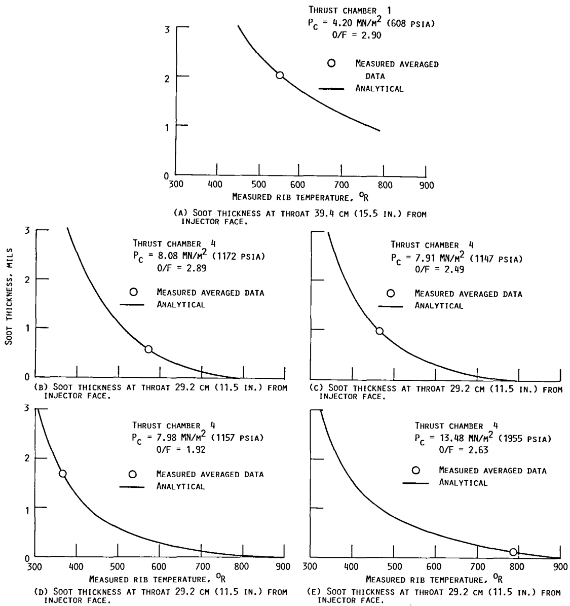
FIGURE 11.- SOOT THICKNESS DISTRIBUTION AT THROAT.
