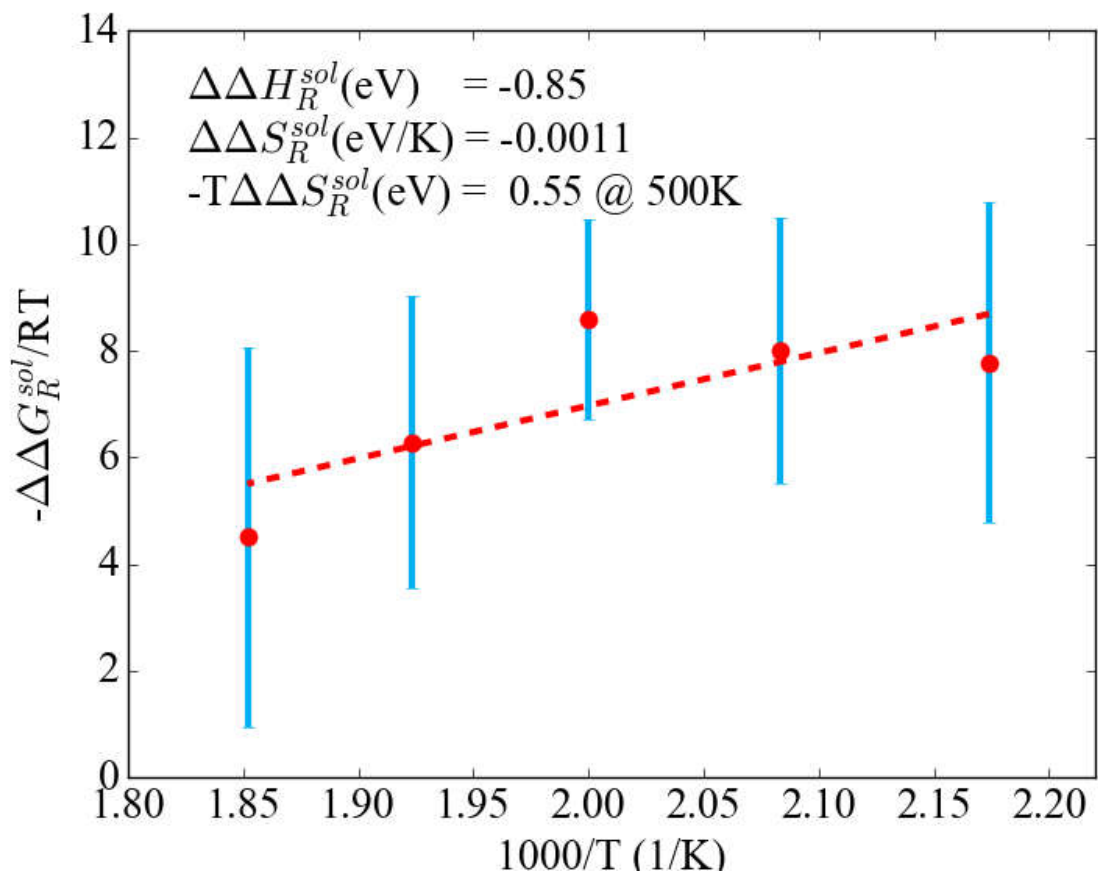
Figure 2.3: Temperature dependence of aqueous solvation effect on the free energy reaction for the primary O-H bond scission of ethylene glycol over a Pt(111) model surface. The error bars indicate 95% confidence interval for the aqueous phase effect on the free energy of the specified reaction.
