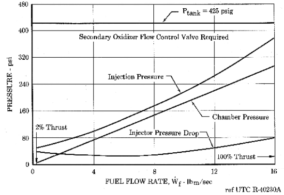
Figure 16. System Pressures versus Fuel Flow Rate with a Constant Secondary Oxidizer Pressure
