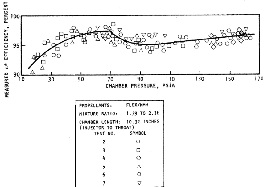
Figure 11. Dual-Manifold Throttling Performance with Series Valve Configuration
