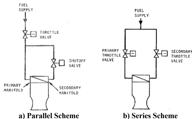
Figure 10. Dual-Manifold Flow Control Schemes
