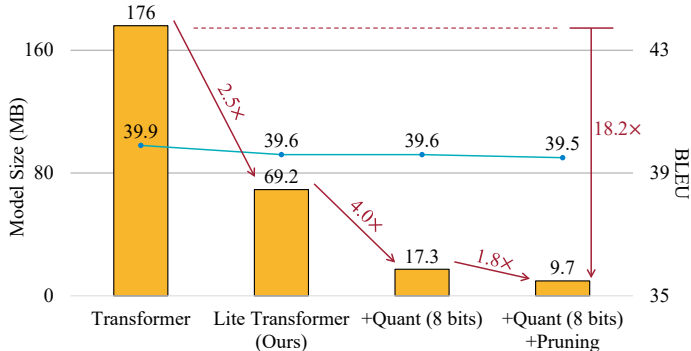
Figure 5: The model size and BLEU score on WMT En-Fr dataset with model compression. Our Lite Transformer can be combined with general compression techniques and achieves 18.2× model size compression. * ‘Quant’ indicates ‘Quantization’.
