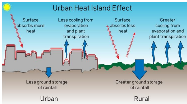
Figure 2: Urban Heat Island
