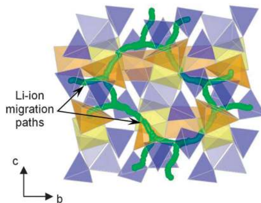
Fig. 9 Calculated paths (green) for long-range Li + migration in Li 2 FeP 2 O 7 involving Li 1 and Li 3 sites viewed perpendicular to the bc plane; simulations involving quasi-2D transport and non-linear pathways. FeO 6 octahedra are shown in yellow, mixed occupancy FeO 5 –LiO 5 units in orange and P 2 O 7 pyrophosphate polyhedra in blue. Reprinted with permission from Wiley Publishers Ltd: Angew. Chem., Int. Ed. (ref. 112). Copyright 2012.
