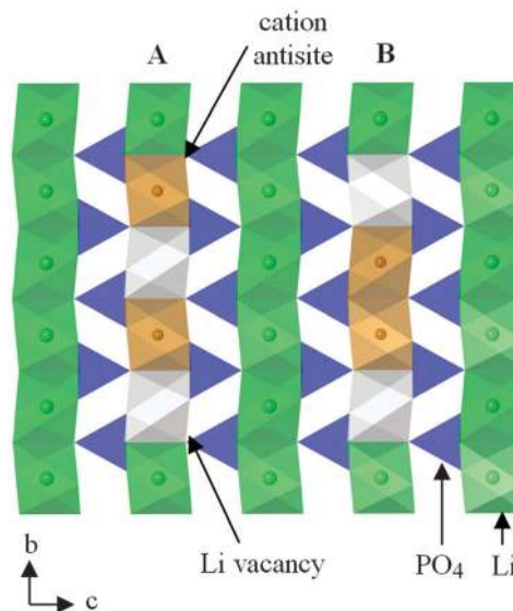
Fig. 10 Schematic of a structural plane of \text{LiFePO}_4 containing two neutral defect cluster arrangements comprised of two antisite defects (Fe on Li sites) and two Li vacancies within b -axis channels: (A) antisite cation and Li vacancy on alternating sites; (B) antisite cations on adjacent sites. Reprinted with permission from ref. 121. Copyright 2010 American Chemical Society.
