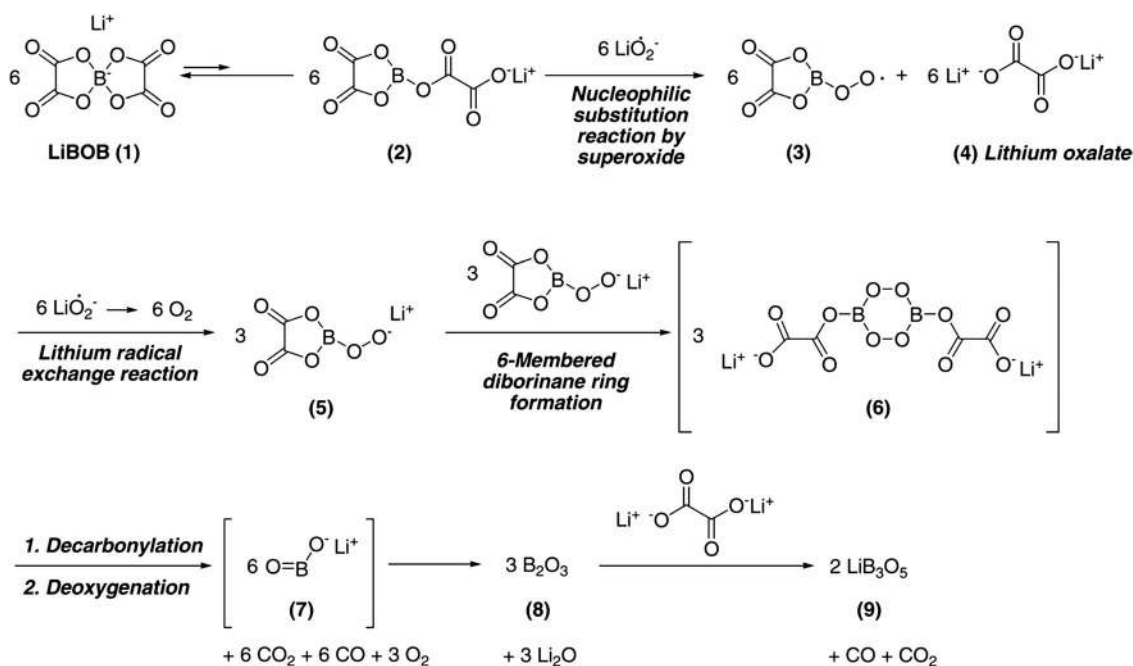
Fig. 7 Proposed mechanism for decomposition of LiBOB by superoxide radicals, obtained from Hyoung Oh et al. 170
