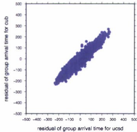
Figure 3. Scatter plot of the residual of group arrival time for ucscd and cub data set at 20 mHz .
