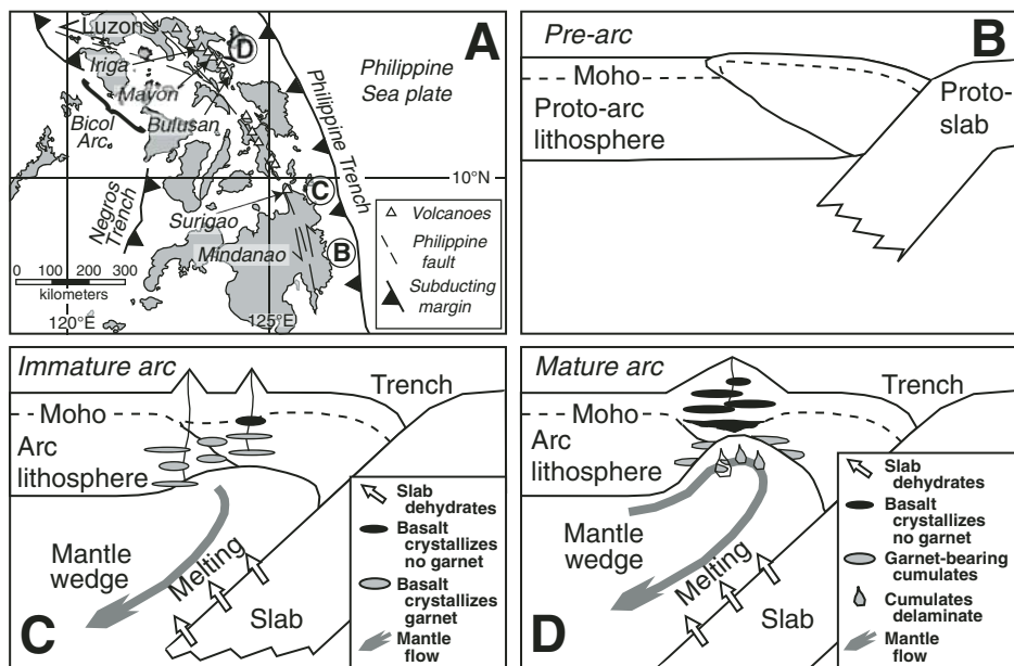
Figure 1. A: East Philippine Arc (EPA) showing location of volcanic centers discussed. Circled letters refer to schematic cross-arc sections in panels B–D, which illustrate thinning of East Philippine Arc lithosphere and its role in determining differentiation depth in nascent, induced subduction zone. B: Pre-arc: subduction of Philippine Sea plate has begun beneath amalgamated proto-arc lithosphere but magmatism has not. C: Immature arc: upwelling of basaltic magma is impeded by lithospheric mantle, and so differentiation occurs beneath Moho, generating garnet-rich cumulates (gray). D: Mature arc: erosion of lithospheric mantle leads to basalt differentiation at shallower levels (black) with garnet-free assemblage. Earlier-formed, garnet-bearing cumulates may return to mantle via lithosphere erosion as mantle flow develops and mantle lithosphere is eroded.
