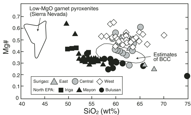
Figure 3. Mg# (Mg/[Mg + Fe]) versus SiO 2 for East Philippine Arc (EPA) lavas. Fields are shown for various estimates of bulk continental crust (BCC; Kelemen, 1995) and for low-MgO garnet pyroxenites from Sierra Nevada (Lee et al., 2006), which represent possible deep-arc cumulates.
