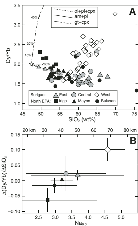
Figure 2. A: Dy/Yb versus SiO 2 for East Philippine Arc (EPA) lavas (data sources in text). Correlations with SiO 2 indicate that differentiation is primary control on Dy/Yb, which increases when garnet crystallizes and decreases when garnet is absent. Differentiation models (showing % crystallization) are from Davidson et al. (2007). gt—garnet; ol—olivine; pl—plagioclase; cpx—clinopyroxene; am—amphibole B: \Delta(\text{Dy}/\text{Yb})/\Delta\text{SiO}_2 (plotted with 2SE uncertainty) is a proxy for mean differentiation depth of each suite and is determined from linear regression of slopes in panel A. This is compared with Na 6,0 , which Plank and Langmuir (1988) showed to be a proxy for crustal thickness, as illustrated on top axis, using 21 arcs worldwide. Uncertainty for Na 6,0 is 95% confidence limit on regression of Na 2 O versus MgO to 6 wt% MgO.
