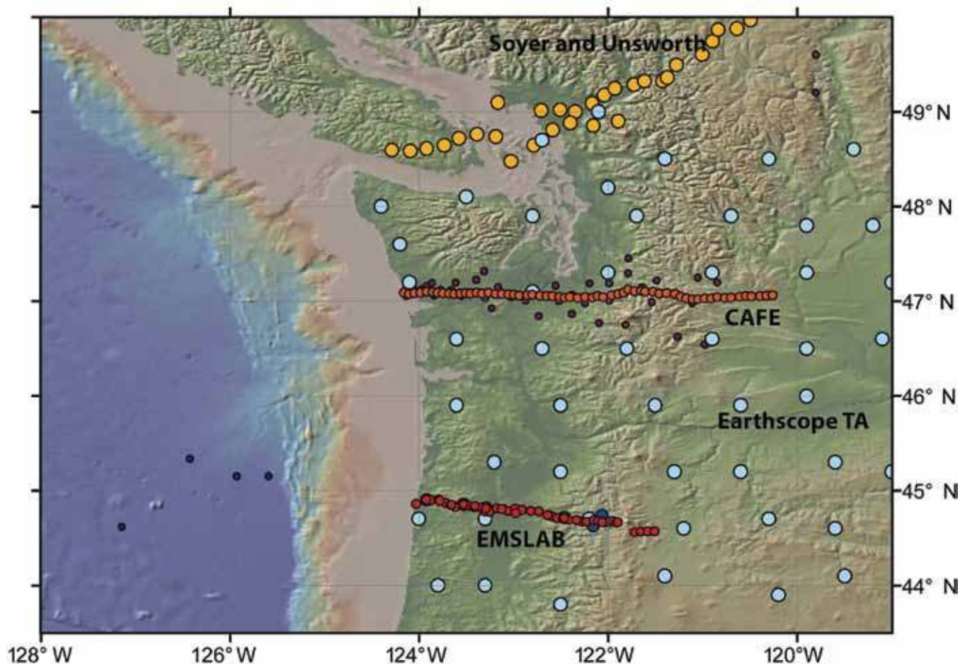
Figure 1. MT transect site distribution for the EMSLAB Lincoln Line (south) and the new Café-MT transect to the north. EMSLAB line contains 40 land sites plus seven sea-floor soundings (5 MT, 2 tipper only; see Wannamaker et al., 1989, JGR). Café line contains 60 wideband site; long-period sites are to be collected summer-fall of 2010.
