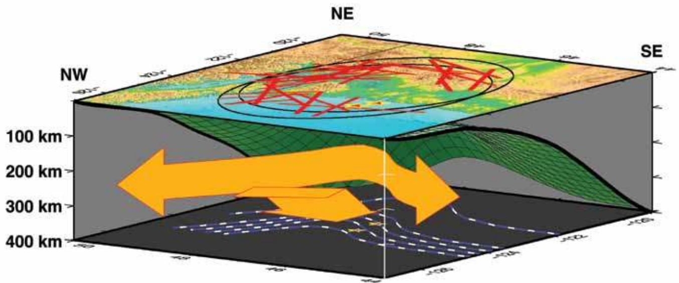
Block diagram showing Juan de Fuca slab geometry (green meshed surface), and top-of-slab depth contours (heavy blue dashed lines, bottom). Source side S splitting measurements are compatible with presence of two anisotropic layers beneath the Juan de Fuca slab: a layer immediately beneath the slab which is characterized by trench-parallel fast shear azimuths, and a deeper layer with fast shear trends parallel to the motion of the Juan de Fuca plate with respect to assumed fixed hotspots (Gripp and Gordon, 2003). Orange arrows schematically show the anisotropy and possibly upper mantle flow directions in these two layers.
