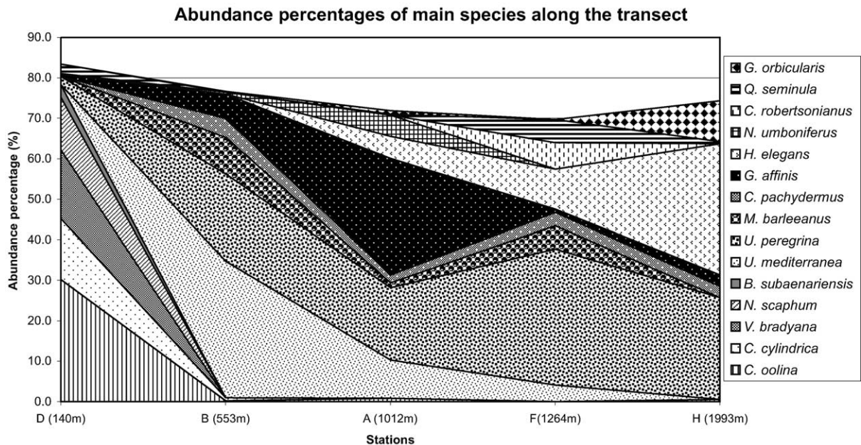
Fig. 9. Composition of the benthic live foraminiferal faunas (in % of the total fauna).
