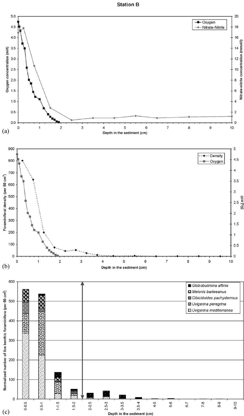
Fig. 4. Station B; (a) dissolved oxygen, and concentration of nitrate + nitrite; (b) dissolved oxygen profile and foraminiferal density (standardised for a 50 cm 3 sediment volume); (c) foraminiferal distribution (number of individuals found in each level, standardised for a 50 cm 3 sediment volume); double arrow represents zero oxygen boundary.
