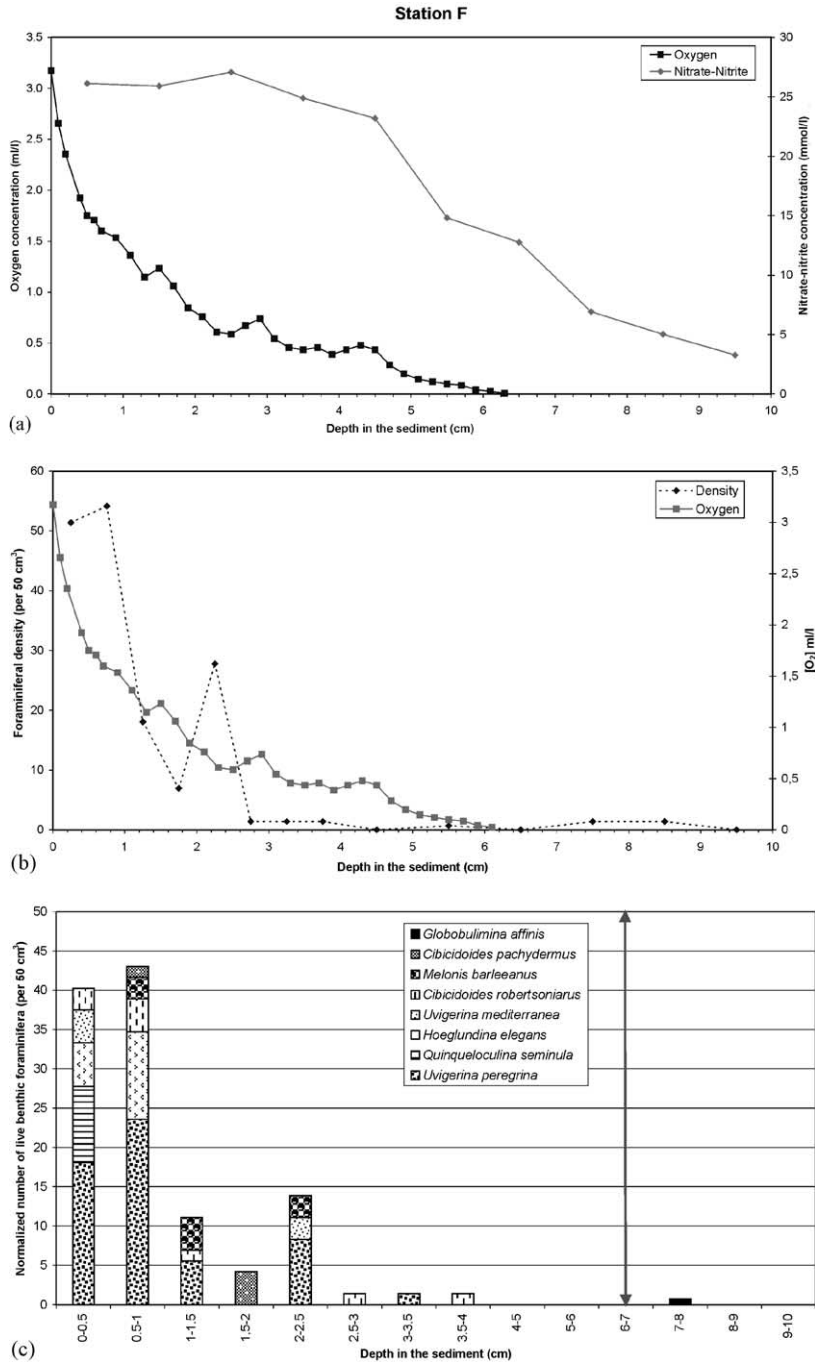
Fig. 6. Station F; (a) dissolved oxygen, and concentration of nitrate + nitrite; (b) dissolved oxygen profile and foraminiferal density (standardised for a 50 cm 3 sediment volume); (c) foraminiferal distribution (number of individuals found in each level, standardised for a 50 cm 3 sediment volume); double arrow represents zero oxygen boundary.
