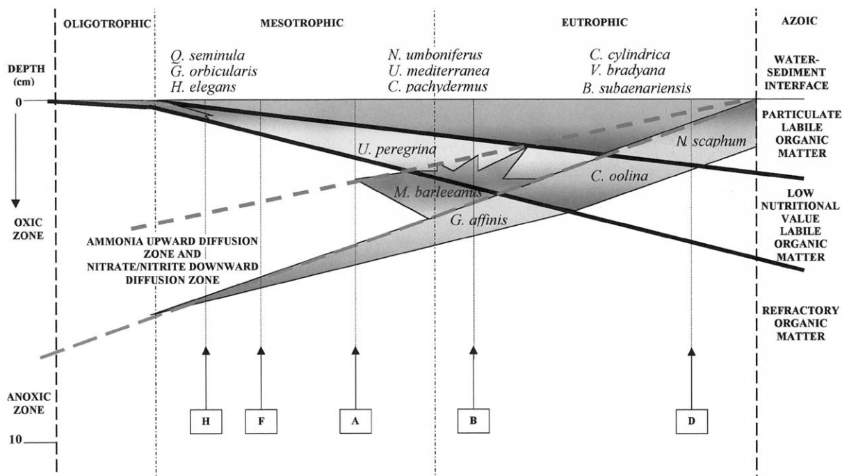
Fig. 11. Microhabitat distribution and specific foraminiferal composition along the bathymetric transect in the Bay of Biscay; the approximate position of our five stations are indicated; see text for full explanation.
