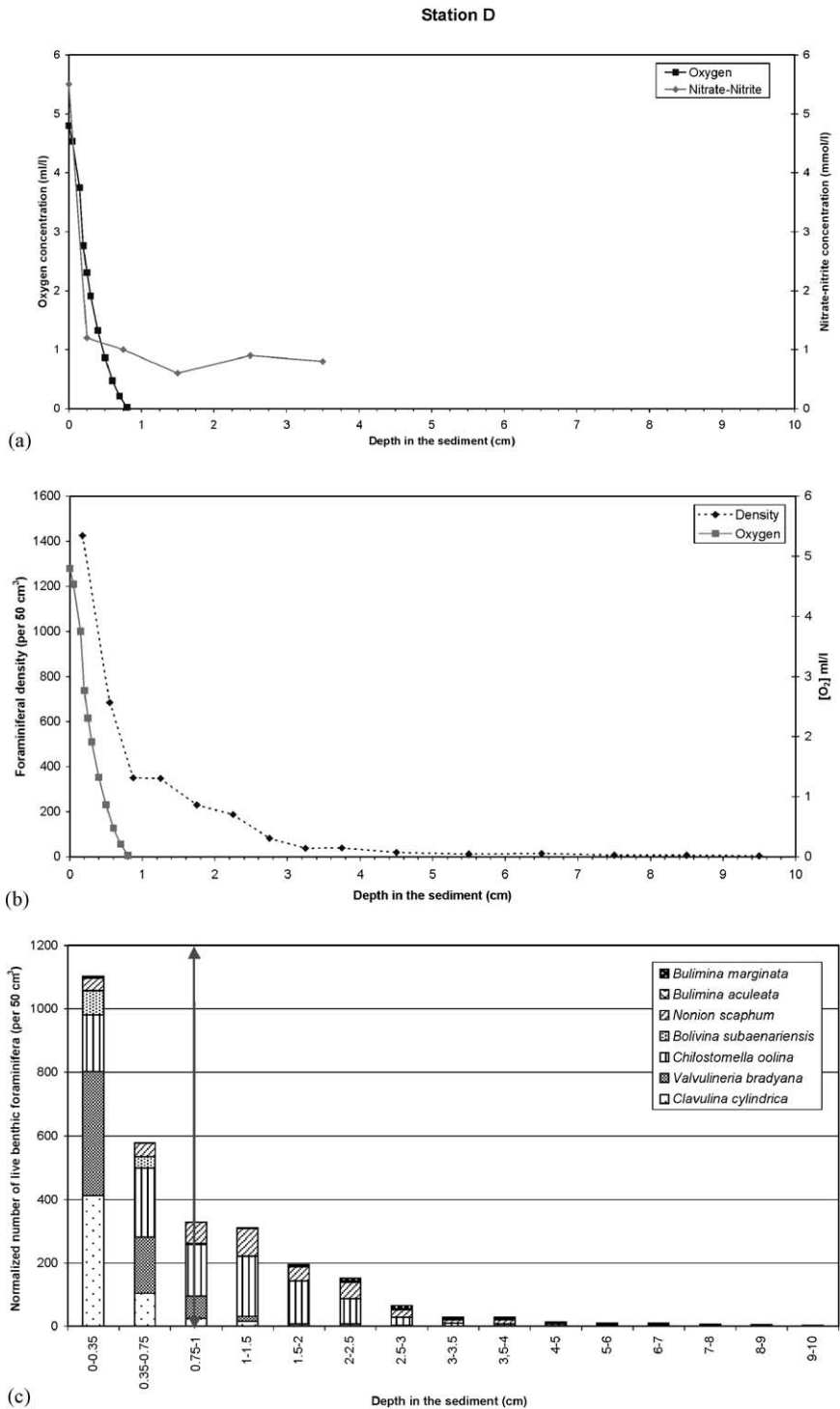
Fig. 3. Station D; (a): dissolved oxygen, and concentration of nitrate + nitrite; (b) dissolved oxygen profile and foraminiferal density (standardised for a 50 cm 3 sediment volume); (c) foraminiferal distribution (number of individuals found in each level, standardised for a 50 cm 3 sediment volume); double arrow represents zero oxygen boundary.
