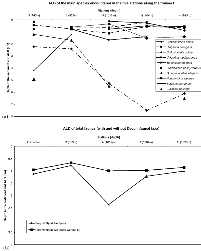
Fig. 8. (a) ALD 10 of the main taxa along the bathymetric transect; (b) ALD 10 of the total faunas (with and without deep infaunal taxa (DI)).
