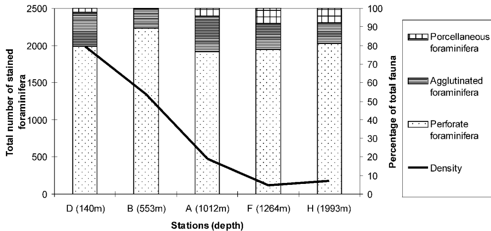
Fig. 2. Abundance of the three main foraminiferal groups, and the density of foraminiferal faunas (total number of stained foraminifera per core (720 cm 3 )) along the bathymetrical transect.
