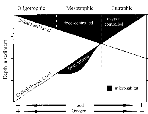
Fig. 10. TROX-model (Trophic condition and Oxygen concentration) explaining the vertical distribution of foraminifera in the top cm of the sediment (after Jorissen et al., 1995); see text for full explanation.
