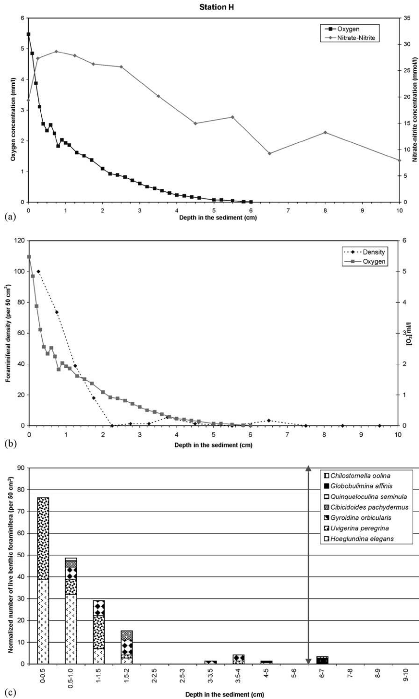
Fig. 7. Station H; (a) dissolved oxygen, and concentration of nitrate + nitrite; (b) dissolved oxygen profile and foraminiferal density (standardised for a 50 cm 3 sediment volume); (c): foraminiferal distribution (number of individuals found in each level, standardised for a 50 cm 3 sediment volume); double arrow represents zero oxygen boundary.
