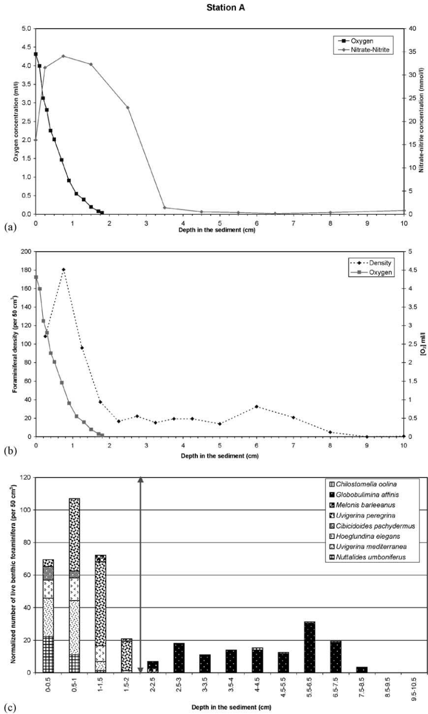
Fig. 5. Station A; (a) dissolved oxygen, and concentration of nitrate + nitrite; (b) dissolved oxygen profile and foraminiferal density (standardised for a 50 cm 3 sediment volume); (c) foraminiferal distribution (number of individuals found in each level, standardised for a 50 cm 3 sediment volume); double arrow represents zero oxygen boundary.
