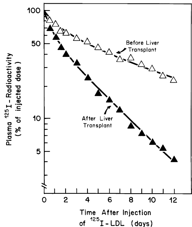
Figure 3. Plasma Decay Curves after Intravenous Injection of 125 I-LDL in the Patient before and after Liver–Heart Transplantation.
