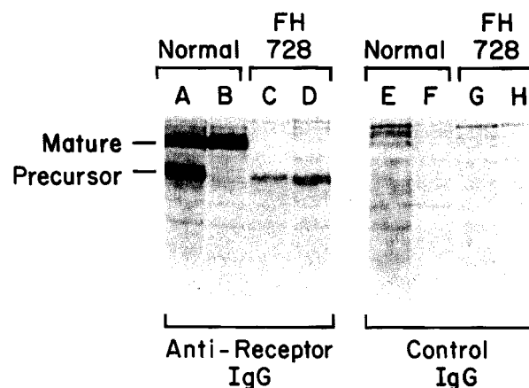
Figure 1. Kinetics of Processing of LDL Receptors in Fibroblasts from a Normal Subject and Patient FH 728.
