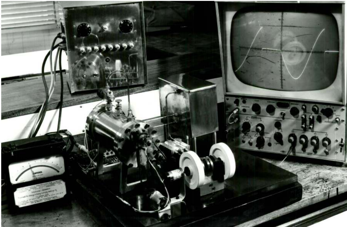
Figure 4: Abe Mamdani and Sedrak Assilian's steam engine, QMC, 1974
