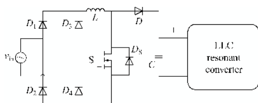
Fig. 9 LED driver of Boost PFC + LLC resonant converter
