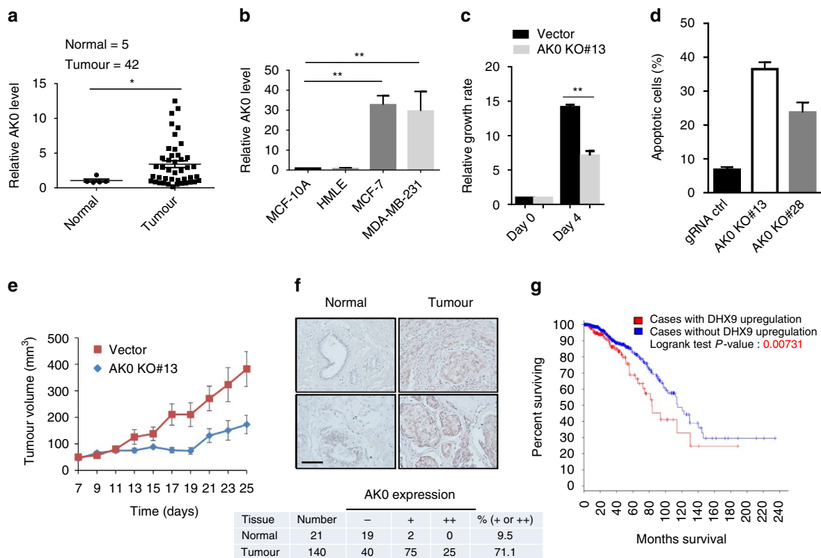
Figure 6 | Upregulation of AK023948 in breast cancer and promotion of tumorigenesis. (a) Detection of AK023948 in the OriGene breast cancer tissue cDNA array by qPCR. (b) AK023948 is upregulated in breast cancer cells (MCF-7 and MDA-MB-231) as compared with non-malignant breast cells (MCF-10A and HMLE). (c) AK023948 KO suppresses cell proliferation of MCF-7, as detected by MTT assay. (d) AK023948 KO promotes apoptosis. Cells were seeded in slide chambers, and treated with H 2 O 2 at 0.8 mM for 4 h before TUNEL assay. Apoptotic cells were counted from three different fields, and apoptotic cell ratio was calculated against total cells. (e) Tumour growth for vector control and AKO KO#13 in nude mice. (f) Expression of AK023948 in breast cancer TMAs, as detected by ISH. Scale bar, 100 \mu m. Bottom: quantitative analysis of AK023948 expression based on the results from f. (g) Upregulation of DHX9 expression is associated with poor patient survival. About 20.9% (229 of 1091 cases analysed) are positive for DHX9 using the Onco Query Language (OQL; EXP>1.5). Values in b,c are s.e.m. ( n = 3). ** P < 0.01 by two-tailed Student's t -test.
