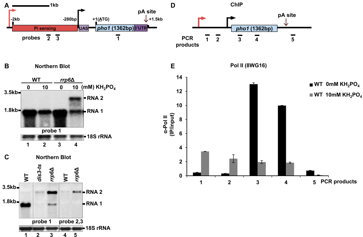
Figure 1. Two overlapping transcripts are made at the pho1 locus. (A) pho1 schematic. The coding sequence is depicted in blue, the upstream activating sequence (UAS) is in purple, the phosphate sensing region is in red, and the 3' UTR is in dark purple. Probes are shown as black bars. (B) Northern blot analysis of RNA isolated from wild-type (WT) and rrp6Δ strains grown in EMMG medium with 0 or 10 mM KH 2 PO 4 . (C) Indicated strains were grown in YES for Northern blot analysis. (D) pho1 schematic showing locations of the PCR products from E. (E) Pol II ChIP experiments performed in wild-type cells grown in EMMG (0 or 10 mM KH 2 PO 4 ). Quantification of the results from three independent experiments is shown; the error bars indicate the standard error. See also Supplemental Figure 1.
