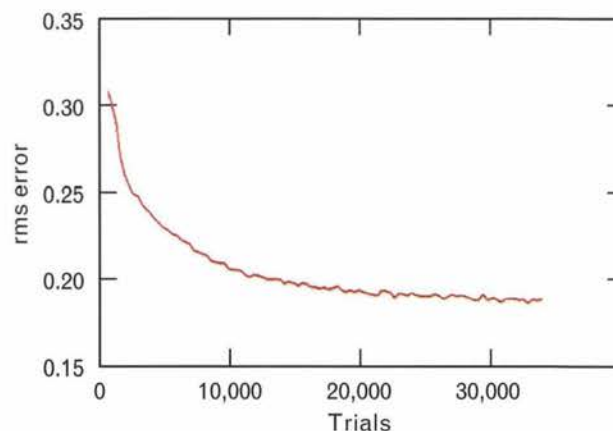
FIGURE 10. Plot of rms error during training for the vowel-classification experiment of Figure 8.
