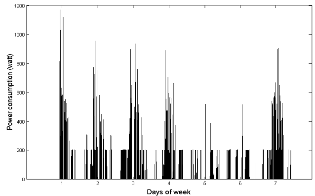
Fig. 5. Pre-processed (energy consumption feature) data of coffee machine for a week.
