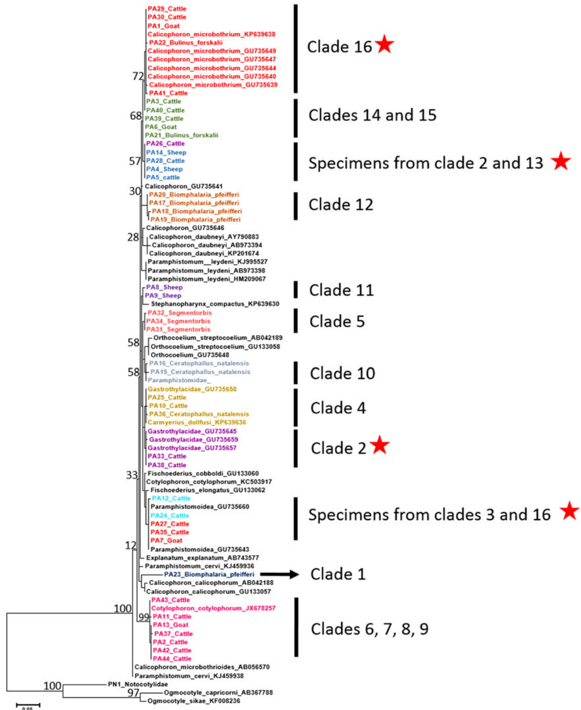
Fig. 2. Phylogenetic relationships of 44 samples of paramphistomoids from this study and from GenBank based on ITS2 (385 bp) sequences inferred from ML (bootstrap values) analysis. Specimens are named based on sample name, the host it was collected from, and colour coded based on clade designation from cox1 distance values. A red star represents clades where we have found evidence of putative hybrids. Adjacent to these indicated clades, are clade numbers that correspond to the same specimens and clade numbers as appearing on the cox1 tree (Fig. 1).
