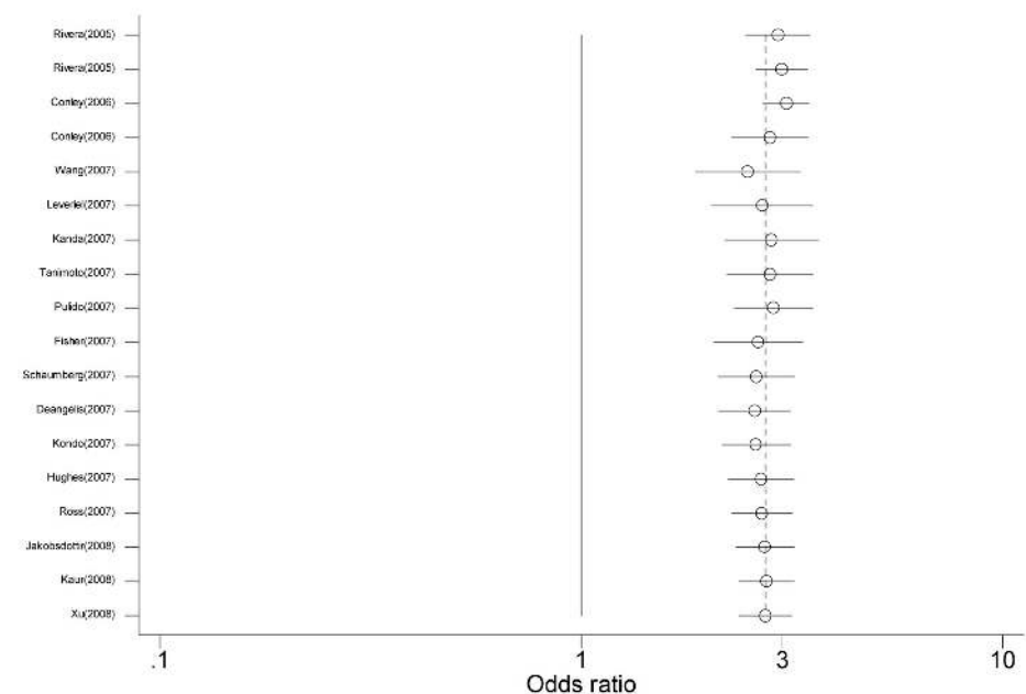
Figure 3. Cumulative random-effects meta-analysis of allele (G versus T) of the LOC387715/ ARMS2 gene rs10490924 G→T polymorphism and age related macular degeneration (AMD). For study details, see Table 4.
