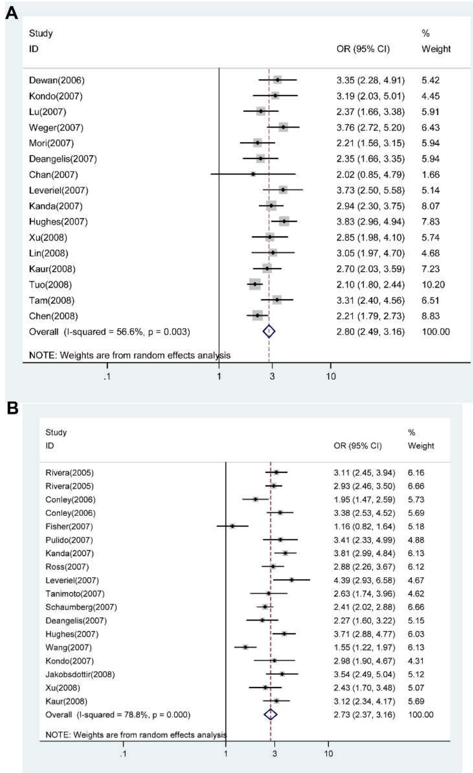
Figure 1. Random-effects meta-analysis of allele (A versus G) of the HTRA1 gene rs11200638 G→A polymorphism and age related macular degeneration (AMD). A: Results from random-effects meta-analysis of allele (A versus G) of the HTRA1 gene rs11200638 G→A polymorphism and AMD. B: Results of the random-effects meta-analysis of the allele (T versus G) of the LOC387715/ARMS2 gene rs10490924 G→T polymorphism and AMD. Reference numbers are given in parentheses. For study details, see Table 1 and Table 2.
