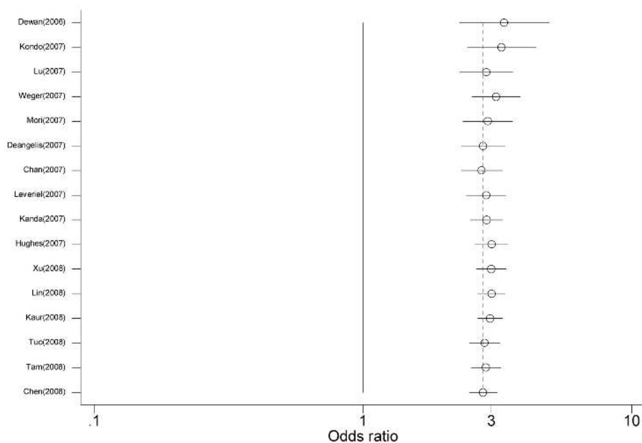
Figure 2. Cumulative random-effects meta-analysis of allele (A versus G) of the HTRA1 gene rs11200638 G→A polymorphism and age related macular degeneration (AMD). For study details, see Table 3.
