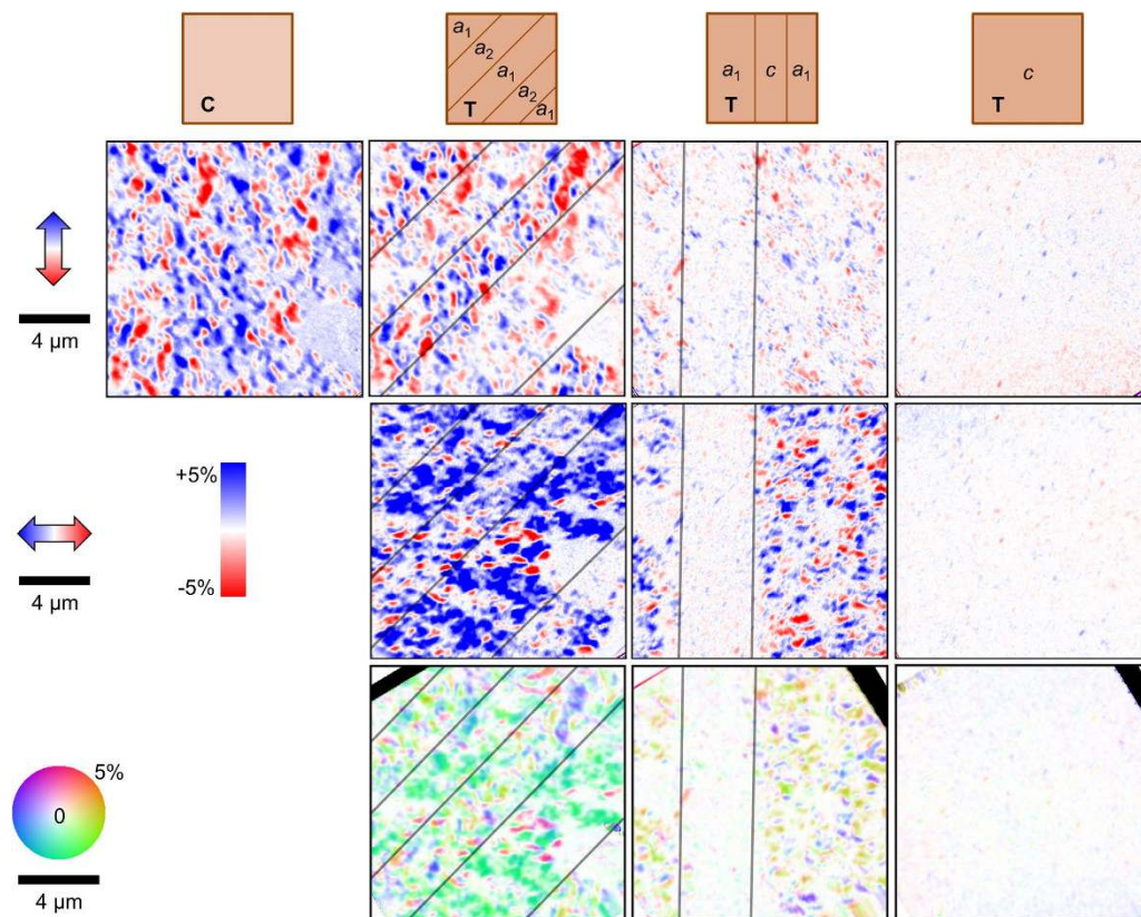
Figure 3. XMCD on various BTO domain arrangements. From top to bottom: sketches of expected BTO domains with reference to Fig. 1(b); corresponding Fe-XMCD images at azimuthal angle 0^\circ with incident X-rays along page vertical; Fe-XMCD images at azimuthal angle 90^\circ with incident x-rays along page horizontal; in-plane XMCD vector maps. Black lines mark inferred ferroelastic domain wall locations. Double-headed red-white-blue arrows indicate the component of magnetization that is measured in each row.
