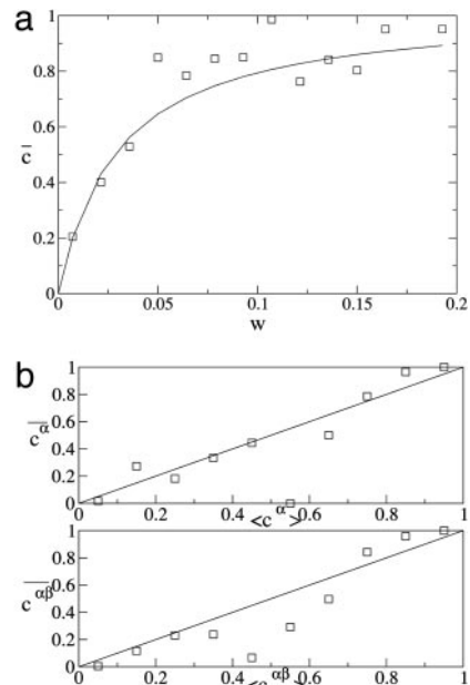
Fig. 3. Statistics of motif ensembles. (a) Testing the statistical model for single subgraphs (Eq. 5 ). Nontree-like subgraphs are enumerated and node pairs i, j are binned according to w_{ij} . The fraction of such pairs carrying a link is shown against w_{ij} . The solid line results from fitting the model with enhanced number of links (Eq. 5 ) to these data, giving \sigma = 3.8 . (b) Testing the statistical model for alignments (Eq. 8 ). (Upper) The average value of c_{ij}^\alpha over all \alpha, i, j with a given expectation value of c_{ij}^\alpha according to Eq. 8 at \sigma = \sigma^* = 3.8 and \mu = \mu^* = 2.25 against the corresponding expectation value ( \square ). For a perfect fit between model and data a straight line is expected (shown solid). (Lower) The same procedure is used averaging the two-point function c_{ij}^\alpha c_{ij}^\beta over all \alpha, \beta, i, j with a given expectation value \langle c_{ij}^\alpha c_{ij}^\beta \rangle .
