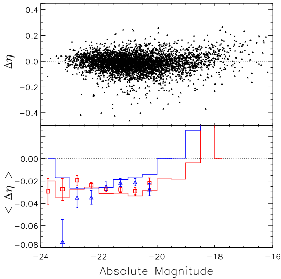
Figure 1. top: The scatter of the \eta - M_I relationship, where \gamma = 0.12 Bottom: The mean \Delta\eta in .5 magnitude bins of the raw distribution (recall that \eta = \log(W) ). The red is for galaxies with cz > 5000 km/s, while the blue is for cz < 5000 km/s. Note the change where M_I > -20 , and also how the red and blue curves appear to have different TF relations. The histograms are for the raw data, with no flow model, while the points, with 1\sigma error bars, are the mean values of \eta - M_I after the fit. The nearby and more distant galaxies now have identical TF relations.
