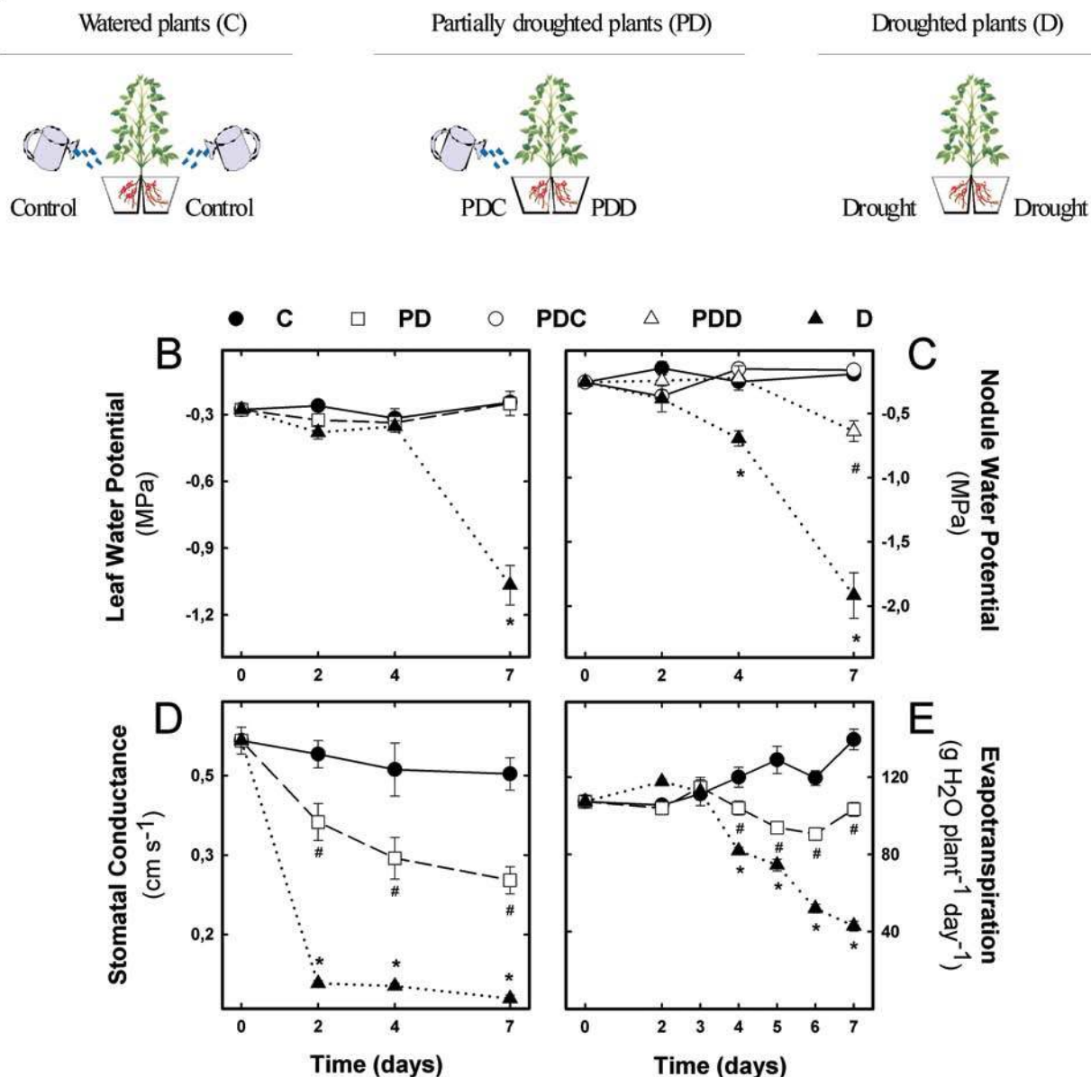
Fig. 1. (A) Schematic representation of the split-root experimental system. (B–E) Effect of partial drought on leaf water potential (B), nodule water potential (C), stomatal conductance (D), and evapotranspiration (E). In B, D, and E, PD denotes partial drought and in (C) both root parts of PD are represented independently: PDC denotes the watered side and PDD the unwatered fraction. Asterisks indicate significant differences (Student's t -test, P \leq 0.05 ) between D and C treatments; hash indicates significant differences between PDD and C plants. Values are mean \pm SE ( n = 3 for B–D; n = 9 for E) (this figure is available in colour at JXB online).
