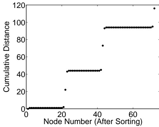
Figure 13: Row Distances for Ideal graph 2. Generated using the membership matrix shown in Figure 12.
