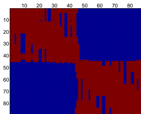
Figure 16: Membership matrix for Ideal graph 3, \alpha = 0.87 .
