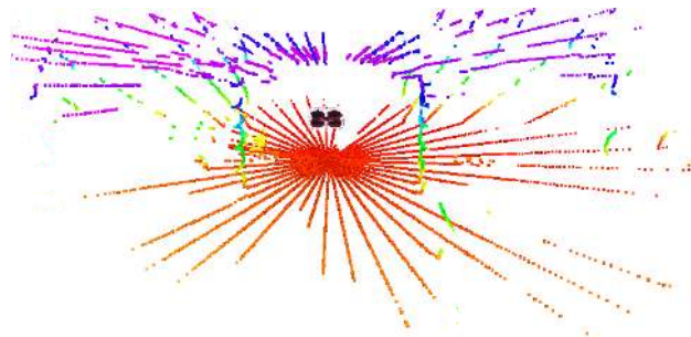
Fig. 3: Indoor 3D scan acquired with our continuously rotating laser scanner. Color encodes height.
