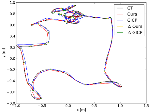
Fig. 7: Absolute trajectory error of the scan registration using the multi-resolution map. Points of the trajectory are projected on the xy -plane.
