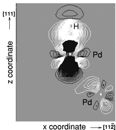
FIG. 4. Charge density difference plot for hydrogen adsorption at the on-top position of two Pd overlayers on Au(111). White contours correspond to charge accumulation while black contours denote charge depletion.
