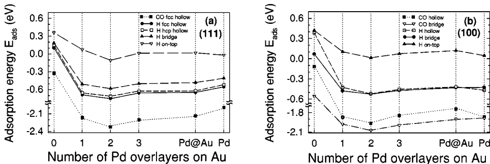
FIG. 2. CO and hydrogen adsorption energies as a function of the number of Pd overlayers on Au for different adsorption sites on the (a) (111) and (b) (100) surface at a coverage of \theta = 0.25 . The pure Pd substrates with the lateral lattice constant of Au ( a = 4.18 \text{ \AA} ) and Pd ( a = 3.96 \text{ \AA} ) are labeled by Pd@Au and Pd, respectively.
