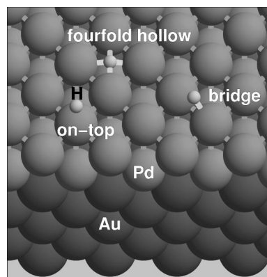
FIG. 1. Considered hydrogen adsorption sites on a two-layer-thick pseudomorphic Pd film on a five-layer slab of Au(100).
