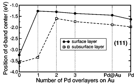
FIG. 3. Position of the local center of the d band with respect to the Fermi energy as a function of the number of Pd overlayers on Au(111) for the surface and the subsurface layer. The overlayers are labeled in the same way as in Fig. 2.
