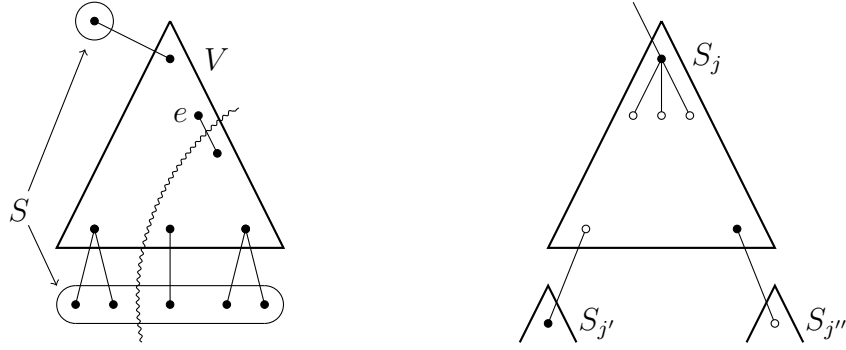
Figure 1: On the left, the edge e splits T[V \cup S] into two trees, partitioning the set S . On the right, a typical subtree S_j ; vertices in color classes 1 and 2 are drawn as white and black circles, respectively. Note that all children of the root of S_j belong to S_j . Since S_{j'} and S_{j''} are below S_j in T_{\Pi} , we have j', j'' > j . Finally, observe that \{S_{j,1}, S_{j,2}\}, \{S_{j,2}, S_{j'',1}\} \in \mathcal{E} .
