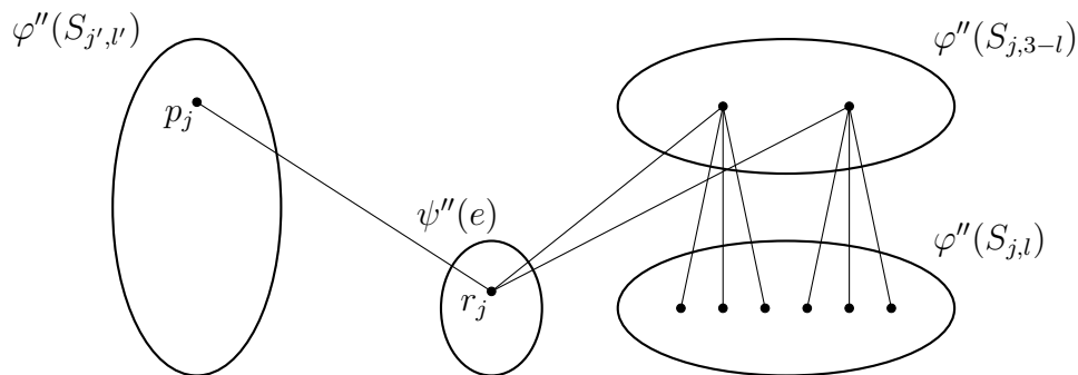
Figure 2: Embedding the subtree S_j into G''
