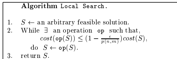
Figure 1: A generic local search algorithm for k -median and facility location problems
