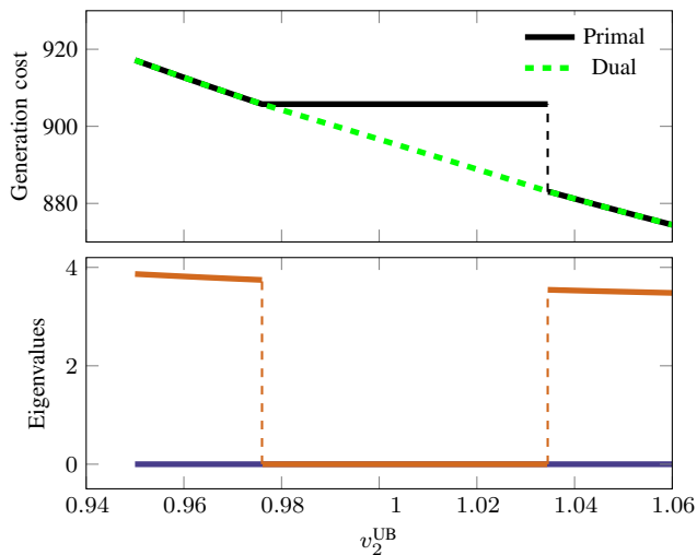
Fig. 8. Performance of SDP optimization method on 2-bus problem.
