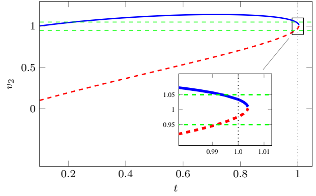
Fig. 2. Alternate load flow solutions as the demand parameter, t , varies.
