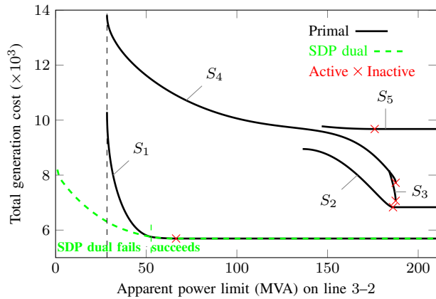
Fig. 9. Primal and dual objectives of the LMBM3 3-bus problem.
