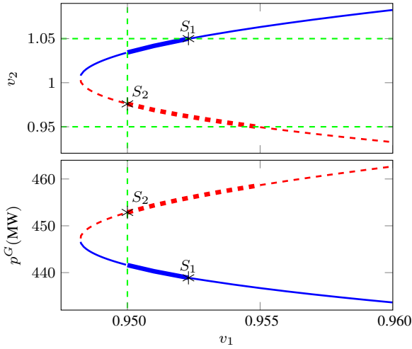
Fig. 3. WB2 2-bus system. Dependency of bus 2 voltage, v_2 , and generator real power p^G on bus 1 voltage v_1 . Feasible region shown by thick lines.
