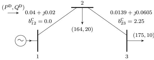
Fig. 4. WB3 3-bus system.
