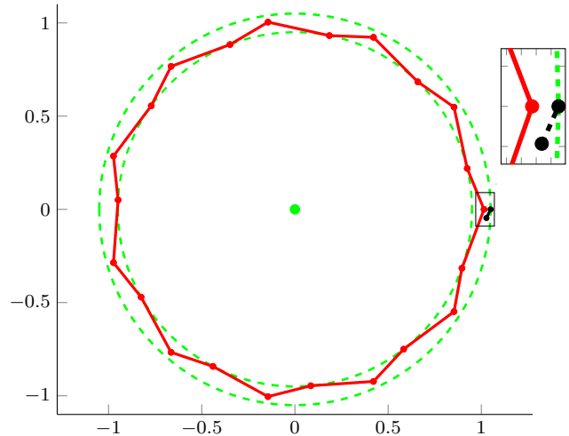
Fig. 7. Real and imaginary voltages (in p.u.) for the 2 solutions of the 22-bus loop case. The loop flow solution has red solid lines and the non loop flow has the black dashed line. The two circles show the \pm 5\% voltage limits.
