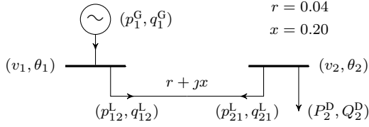
Fig. 1. WB2 2-bus system.
