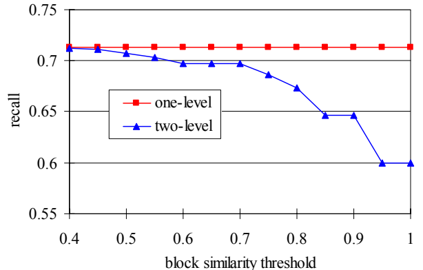
Figure 12: Recall for different block similarity thresholds.
