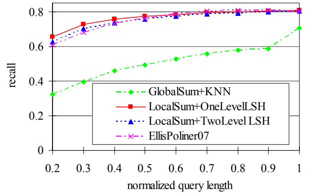
Figure 14: Recall for different query lengths.
