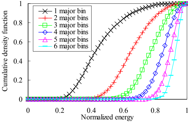
Figure 3: CDF of normalized energy.
