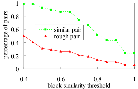
Figure 11: Percentage of matched pairs.
