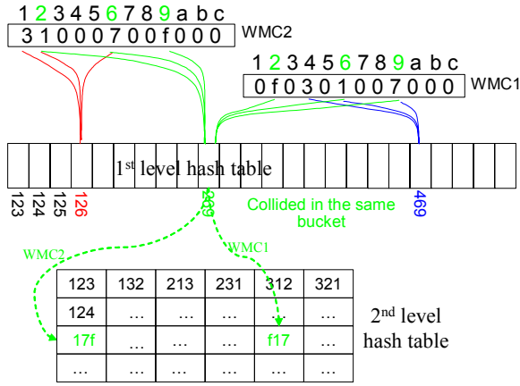
Figure 5: Two-level LSH structure.
