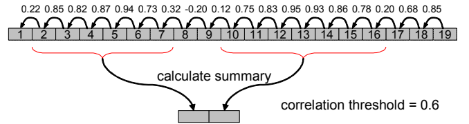
Figure 2: Local summarization.
