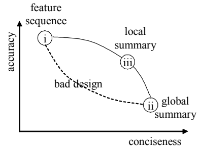
Figure 1: Accuracy-conciseness tradeoff.
