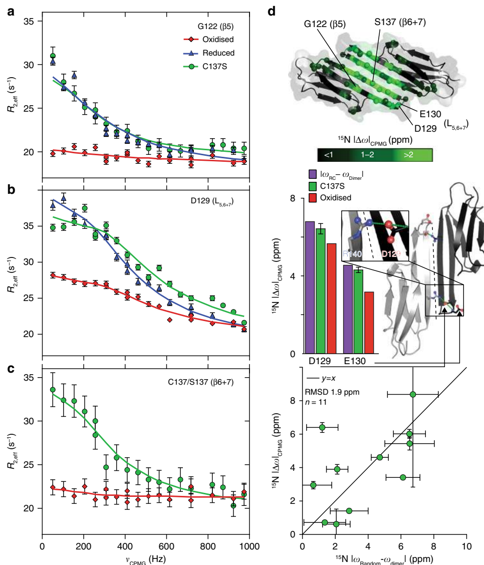
Fig. 5 Relaxation dispersion reveals partial unfolding of the cHSP27 monomer. ^{15}N CPMG RD experiments quantify \mu s–ms motions in oxidised (red), reduced (blue), and C137S (green) cHSP27. Fitted curves from a global analysis are shown as solid lines. Significant CPMG RD curves were observed in the \beta_5 strand ( a ), L_{5,6+7} loop ( b ), and the \beta_6 + 7 strand ( c ). Redox-independent motions were observed in L_{5,6+7} , which arise from unfolding of the loop, whereas only the non-covalent dimers in C137S and reduced cHSP27 show motions throughout \beta_5 and \beta_6 + 7 . d (top) CPMG RD-derived ^{15}N chemical shift changes in C137S ( |\Delta\omega| ) plotted onto the structure (PDB: 4mjh) reveal structural changes in L_{5,6+7} and the \beta_5 and \beta_6 + 7 strands. (middle) The ^{15}N |\Delta\omega| values in L_{5,6+7} are similar in both C137S and oxidised cHSP27, and correlate with those expected for a transition to a random coil, indicating that unfolding of L_{5,6+7} is independent of oxidation state. In L_{5,6+7} , D129 forms an intermolecular salt bridge with R140 from an adjacent subunit, and the amide nitrogen from E130 forms a hydrogen bond with the carbonyl of D129 within the same subunit. All error bars are derived from fitting and represent SD values. (bottom) ^{15}N |\Delta\omega| values in L_{5,6+7} and \beta_6 + 7 upon monomerisation are compared to the changes expected for random coil formation. The agreement is reasonable, indicating the monomer is substantially disordered in these regions. Error bars represent SD values
