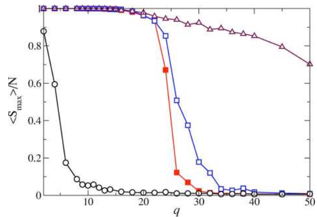
FIG. 8. (Color online) Influence of the interacting field on the nonequilibrium order-disorder transition as described by the order parameter \langle S_{\max} \rangle / N . Results are shown for B=0 (solid squares), a global [ B=10^{-5} (empty squares), B=0.3 (circles)] and a local [ B=10^{-5} (triangles)] field. Parameter value F=3 .
