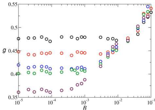
FIG. 6. (Color online) Finite size effects at small values of the strength B of a global field Order parameter g as a function of B is shown for system sizes N=20^2, 30^2, 40^2, 50^2, 70^2 (from top to bottom). Parameter value q=30 .
