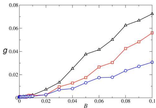
FIG. 2. (Color online) Order parameter g as a function of the coupling strength B of an external (squares), global (circles), and local (triangles) field. Parameter value q = 10 < q_c .
