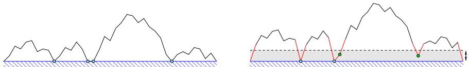
FIG 12. The transformation: A random subset of the pinned sites is unpinned and the height at the corresponding sites is chosen at random in the interval (0, 1) . To avoid overcounting, the whole interface, except the pinned sites, is lifted by 1 before this procedure is applied.
