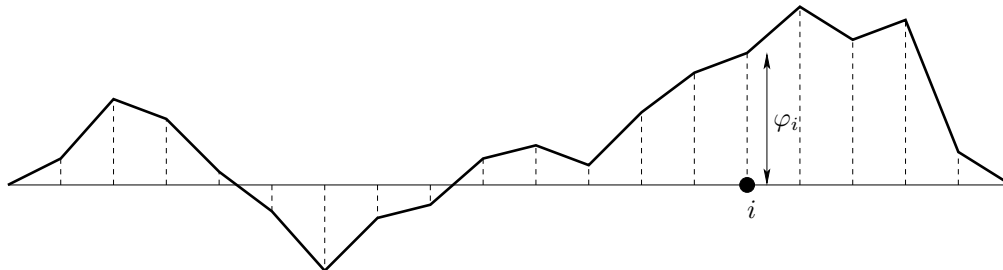
FIG 1. A one-dimensional interface \varphi .
