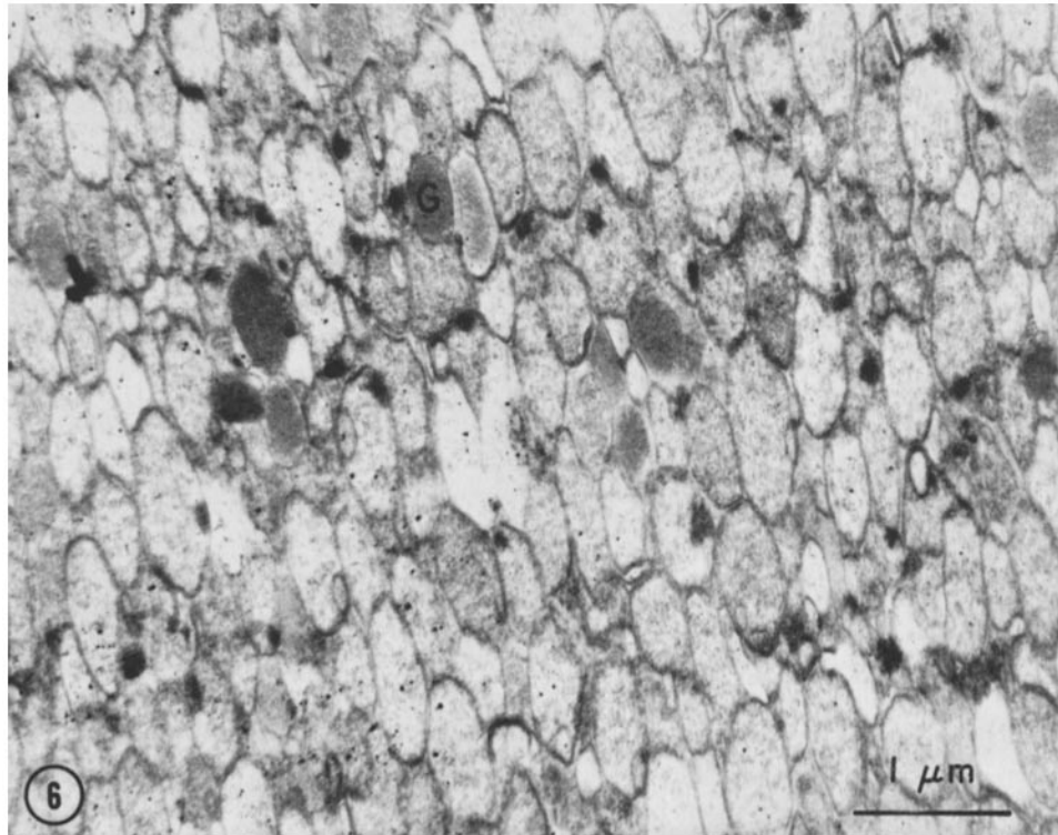
FIGURE 6 Electron micrograph of the glyoxysomal fraction after treatment with 0.2 M KCl. Bar represents 1 \mu m. Section was stained with lead citrate. G, glyoxysome. \times 19,500 .
