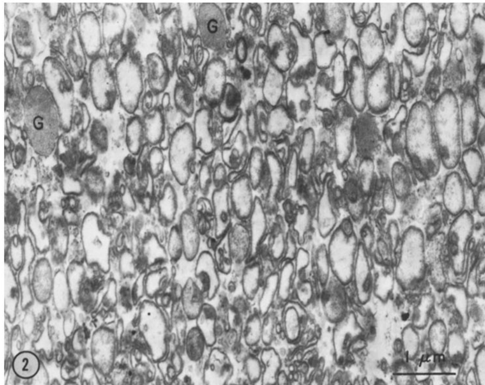
FIGURE 2 Electron micrograph of the glyoxysomal fraction after osmotic shock. The membranes appear intact and the cores, where present, occur inside the ghosts. A few of the glyoxysomes (G) still retained their amorphous matrix. Bar represents 1 μm. Section was stained with lead citrate. × 17,000.
