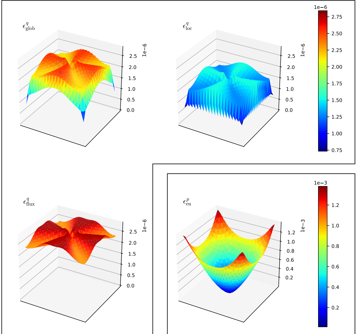
Figure 2: Distribution of \|\epsilon_{\text{glob}}\|_q^q = \|\mathcal{R}\|_{V'}^q , (top left), \|\epsilon_{\text{loc}}\|_q^q = \sum_{\mathbf{a} \in \mathcal{V}_h} \frac{1}{N} \|\mathcal{R}\|_{(V^{\mathbf{a}})}^q , (top right), \|\epsilon_{\text{flux}}\|_q^q = \|\boldsymbol{\sigma}(\nabla u) - \boldsymbol{\sigma}(\nabla u_h)\|_q^q (bottom left), and \|\epsilon_{\text{en}}\|_p^p = \|\nabla(u - u_h)\|_p^p (bottom right) for the case Chaillou-Suri , p = 1.5 , \#\text{cells}=1600
