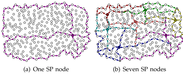
Fig. 7. Information mesh in an arbitrary sensor network
