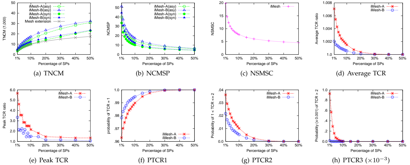
Fig. 9. iMesh in a network of 10, 000 nodes. Abbreviation “asy” (“syn”) indicates the asynchronous (resp., synchronous) nature of the network. The absence of such an abbreviation implies that a metric is irrelevant to network synchrony.
