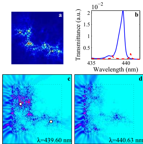
Fig. 3. (Color online) a. Hybridization of four localized states by setting the index of refraction to 2.9 and 2.8 for left and right scatterers, respectively, shown as white spots; all other scatterers set at n_c = 2.0 . b. Transmittance spectra for plane wave impinging from left on perturbed (solid line) and unperturbed (dotted line) systems. c. Field amplitude spatial distribution for wave impinging on perturbed system at \lambda = 439.60 nm. d. Field amplitude spatial distribution for wave impinging on unperturbed system at \lambda = 440.63 nm.
