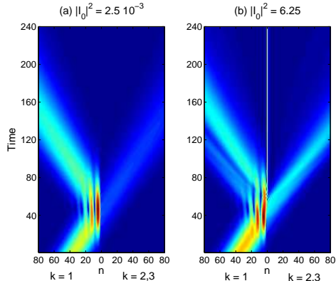
FIG. 7: (Color online) Evolution of a Gaussian pulse scattered by the N = 3 nonlinear junction (a nonlinear Y -splitter), for two different pulse intensities: (a) |I|^2 = 2.5 \times 10^{-3} , and (b) I = 6.25 . Other parameters are: \epsilon_0 = -1 , \lambda = 1 , \sigma = 20 and q_0 = 2.75 . These results should be compared with the results for the plane-wave scattering shown in Fig. 4.
