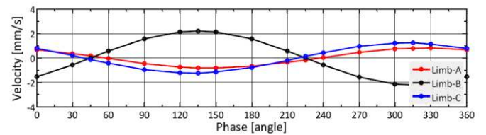
Fig. 17. Comparison of measured variation of instantaneous fundamental velocity (100 Hz) at the centre and half height on each limb during one cycle of magnetisation between centre limb (Limb-B) and outer limbs (Limb-A and Limb-C) at 1.5 T, 50 Hz.
