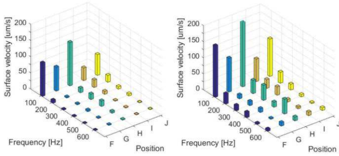
Fig. 12. Variation of RMS values of harmonics of surface velocity [ \mu\text{m/s} ] at locations on the front and side surfaces of the CGO MSL three-phase core magnetized at 1.0 T to 1.7 T, 50 Hz.
