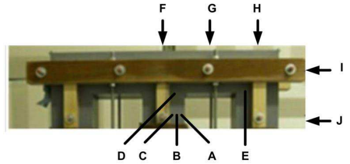
Fig. 9. Positions at which localised vibration was measured on the surface of the three-phase, MSL CGO core
