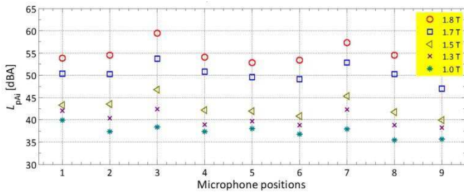
Fig. 8. Variation of averaged (3 trials) A-weighted sound pressure level from microphone placed on the prescribed contour (positions 1 to 8) and above (position 9) of three phase MSL CGO core at flux densities of 1.0 T to 1.8 T, 50 Hz.
