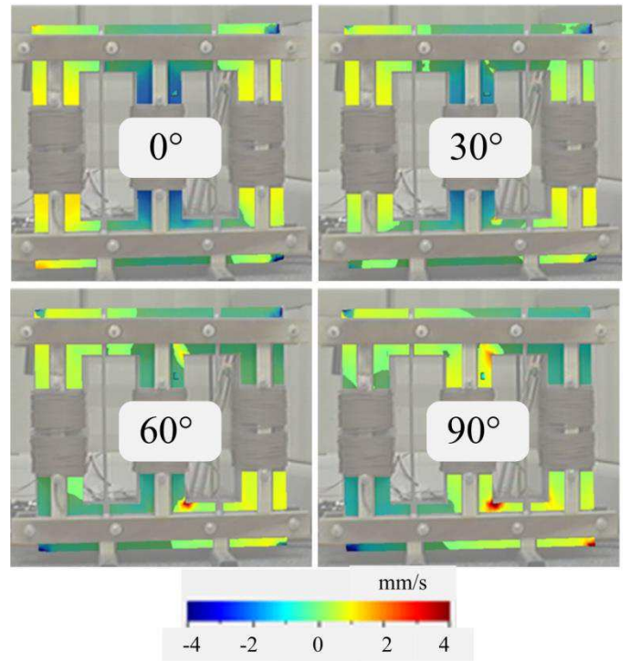
Fig. 16. Measured instantaneous velocity contour on the front surface of the CGO MSL core with clamping pressure of 0.33 MPa at \omega t = 0^\circ, (180^\circ), 30^\circ, 60^\circ, 90^\circ at B_p=1.7 T.
