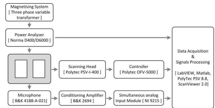
Fig. 2. Overview of the transformer core magnetising method and the noise and vibration measurement process.
