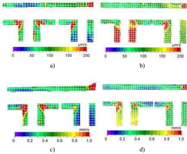
Fig. 18. Distribution of rms value of localised out of plane velocity of the front surface of CGO cores (a) SSL, 1.0 T, (b) MSL, 1.0 T (c) SST, 1.7 T (d) MSL, 1.7 T.
