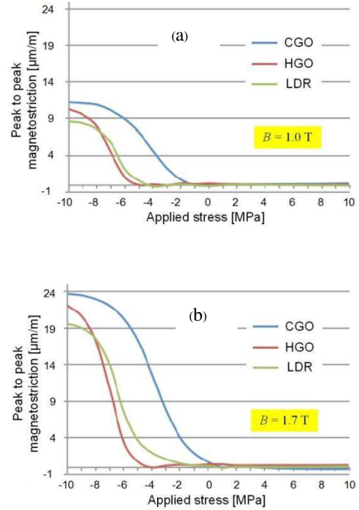
Fig. 1. Stress sensitivity of the peak to peak MS of strips of CGO, HGO and LDR magnetised along their RDs at 50 Hz (a) 1.0 T peak magnetisation, (b) 1.7 T peak magnetisation.
