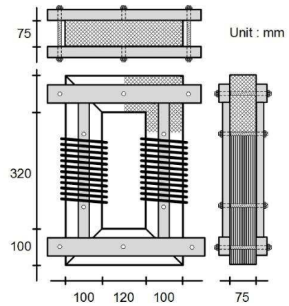
b) Single phase core
