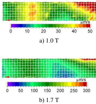
Fig. 13. Distribution of in-plane component of rms velocity ( \mu\text{m/s} ) on the top surface of the CGO, MSL core at (a) 1.0 T, (b) 1.7 T.
