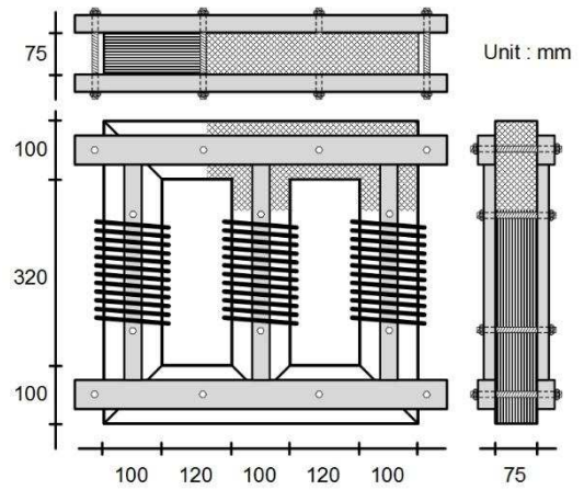
a) Three phase core
