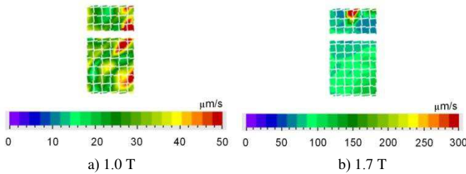
Fig. 14. Distribution of in-plane component of rms velocity ( \mu\text{m/s} ) on the side surface of the CGO, MSL core at (a) 1.0 T, (b) 1.7 T.
