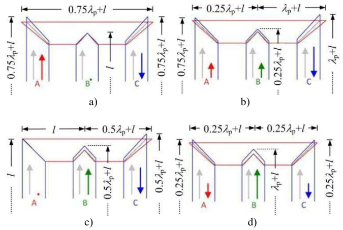
Fig. 15. Representations of magnitude and direction of instantaneous flux density and simulated magnetostrictive distortion at (a) \omega t=0^\circ and 180^\circ (b) \omega t=30^\circ (c) \omega t=60^\circ (d) \omega t=90^\circ
