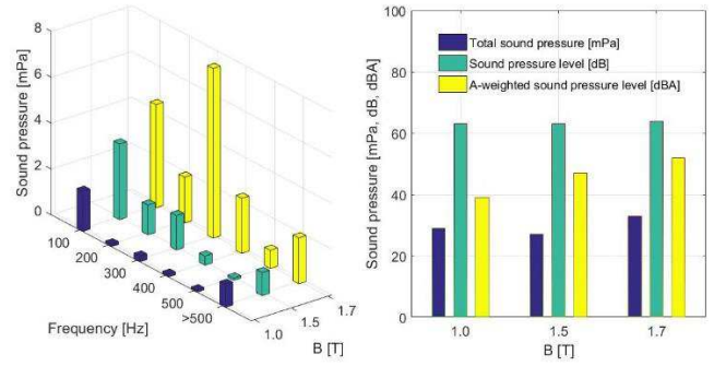
Fig. 10. Harmonics of sound pressure [mPa] emitted from front surface of the three phase CGO core at 1.0 T, 1.5 T and 1.7 T, 50 Hz (detected by microphone 3)
