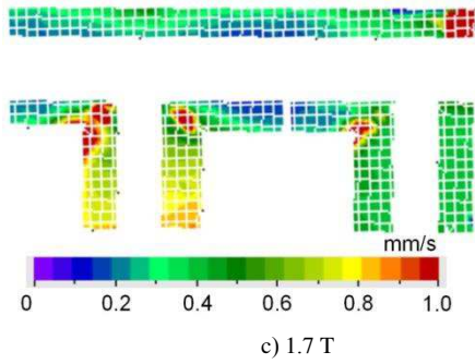
Fig. 11. RMS vibration velocity distribution on the front surface of the CGO MSL core at (a) 1.0 T (b) 1.5 T (c) 1.7 T.
