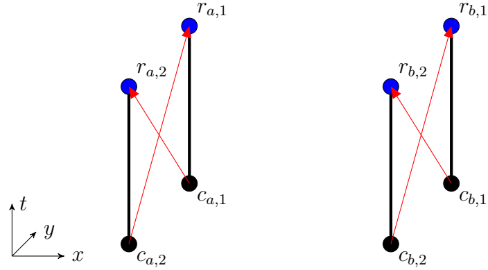
Figure 13: An arrangement of causal diamonds on which we can define an assembly task. Define authorized sets \mathcal{A}_1 = \{D_{a,1}, D_{b,1}\} and \mathcal{A}_2 = \{D_{a,2}, D_{b,2}\} while any set of three or four diamonds is deemed unauthorized. One can check that every unauthorized set has \mathcal{U}_i \setminus \mathcal{A}_j causally connected to \mathcal{A}_j , so theorem 13 gives that this task can be completed. To do so, the initial system A is encoded using the quantum one-time pad and sent towards the pair of diamonds labelled ‘ a ’, D_{a1} and D_{a2} . It should be handed over at whichever diamond receives a call. The key k from the one-time pad is stored in a ((2, 2)) secret sharing scheme as k = k_a \oplus k_b and k_a and k_b are sent towards the ‘ a ’ and ‘ b ’ pairs of diamonds respectively. At the ‘ a ’ pair of diamonds, k_a is returned to D_{a1} if there is a call there and no call at D_{a2} , or at D_{a2} if there is a call there and no call at D_{a1} . The k_b string is returned to D_{b1} or D_{b2} using the same logic. If three or four diamonds receive calls, then at least one of the ‘ a ’ or ‘ b ’ pairs of diamonds will not receive a share of the ((2, 2)) scheme, so Bob will not receive the A system. Notice that the task is possible even though \mathcal{A}_1, \mathcal{A}_2 are subsets of the unauthorized sets, violating the monotonicity requirement of quantum secret sharing.
