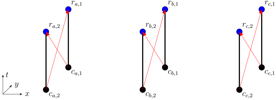
Figure 14: Arrangement of call-reveal pairs used in the proposed party-independent transfer protocol. Bob 1 controls the diamonds D_{a,1}, D_{b,1}, D_{c,1} while Bob 2 controls D_{a,2}, D_{b,2}, D_{c,2} .
