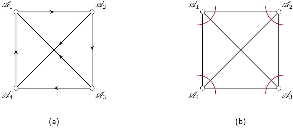
Figure 5: Illustration of the functioning of the error-correcting code used in theorem 6. a) A directed graph that describes the causal connections between the authorized regions of a localize task. In this case the task involves four authorized regions. b) To complete the task, we employ an error-correcting code that associates a share to each edge in the corresponding undirected graph. The encoded qubit can be reconstructed from the shares associated with the edges attached to any one vertex, corresponding to the sets of edges crossed by the purple arcs. For a single logical qubit, the shares on each edge consist of two qubits. A detailed construction of the code can be found in [6], and a more efficient version in [21]. For infinite dimensional versions see [8].
