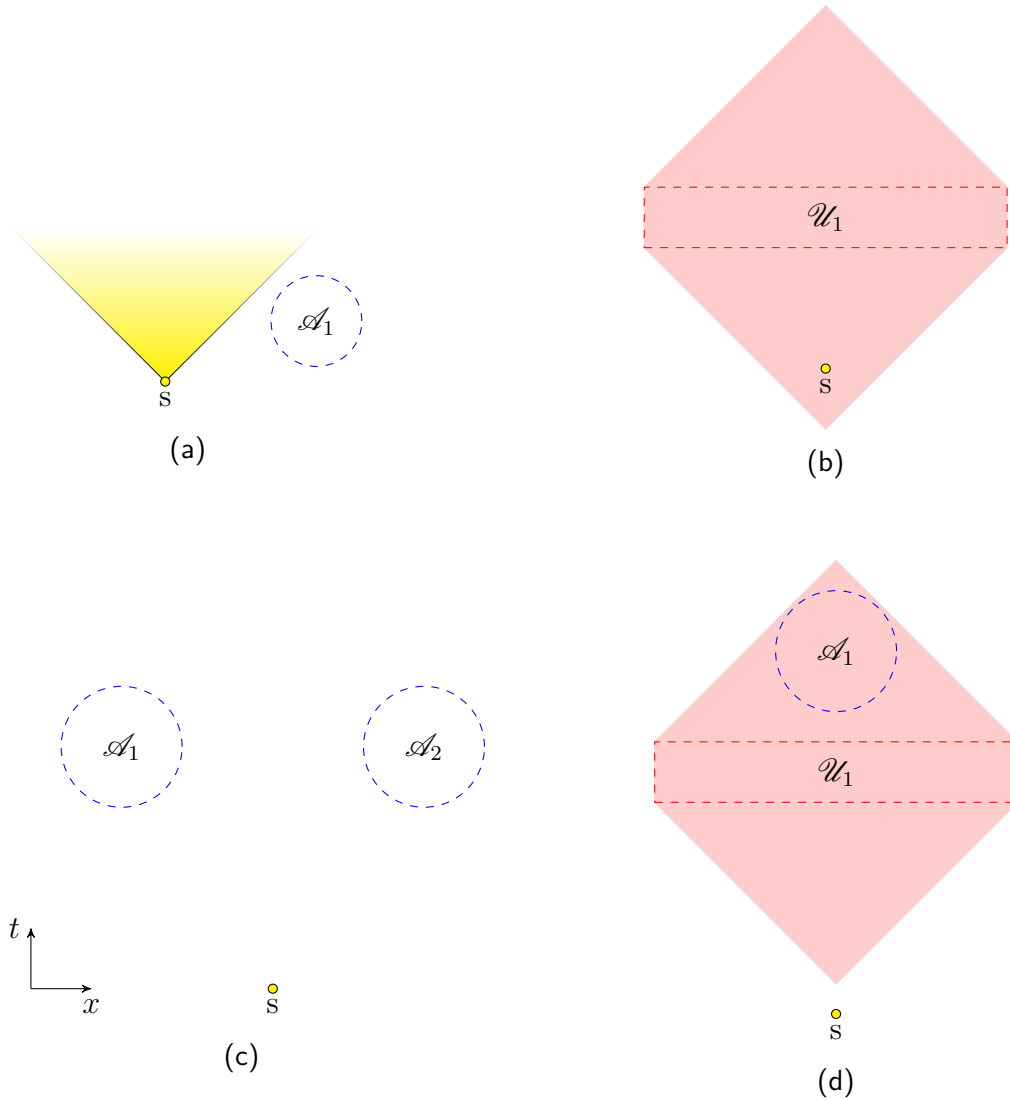
Figure 6: Four impossible localize-exclude tasks: (a) An authorized region is entirely outside the future light cone of s , so system A can't be localized there without violating the no-signalling principle. (b) The initial location of the quantum system is in the domain of dependence of an unauthorized region \mathcal{U}_1 , so can be reconstructed from data in \mathcal{U}_1 . (c) A quantum system cannot be localized to both the spacetime regions \mathcal{A}_1 and \mathcal{A}_2 , due to the no-cloning theorem. (d) A quantum system cannot be localized to \mathcal{A}_1 without passing through the region \mathcal{U}_1 , since there is no causal curve which passes through \mathcal{A}_1 and not \mathcal{U}_1 . The red shaded region indicates the domain of dependence of the unauthorized region \mathcal{U}_1 . The yellow shading indicates the future light cone of the start point.
