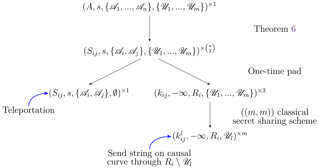
Figure 8: Diagram of the sufficiency proof of theorem 8. In three steps, the proof reduces completing the localization task on the system A with n authorized sets and m unauthorized sets, denoted by (A, s, \{\mathcal{A}_1, \dots, \mathcal{A}_n\}, \{\mathcal{U}_1, \dots, \mathcal{U}_m\}) , to completing \binom{n}{2} instances of (S_{ij}, s, \{\mathcal{A}_i, \mathcal{A}_j\}, \emptyset) on quantum shares, and 3m\binom{n}{2} instances of (k_{ij}^l, -\infty, R_i, \mathcal{U}_l) on classical shares, where the region R_i may be either the start point or an authorized region. The notation -\infty indicates the share is available at early times. The first step in the protocol is to recycle the error-correcting code from theorem 6 to encode the A system into shares S_{ij} . At the second step, the one-time pad is applied to each of the S_{ij} . This allows the unauthorized regions to be avoided by introducing additional classical shares, but without the need for further uses of quantum error-correcting codes.
