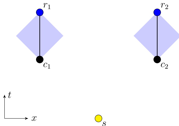
Figure 11: A state-assembly task with two call-return pairs. A call to c_1 is required to result in the system returned at r_1 , and likewise for c_2 and r_2 (indicated by the black lines), while a call to both shouldn't result in more than one copy of the system being turned over. This task is impossible as shown by theorem 11, because r_2 is outside the future light cone of c_1 and r_1 is outside the future light cone of c_2 . In the language of definitions 9 and 10, c_1 and r_1 form a causal diamond D_1 (shown in blue), and the authorized set \mathcal{A}_1 consists of the single diamond D_1 (similarly for c_2 and r_2 ).
