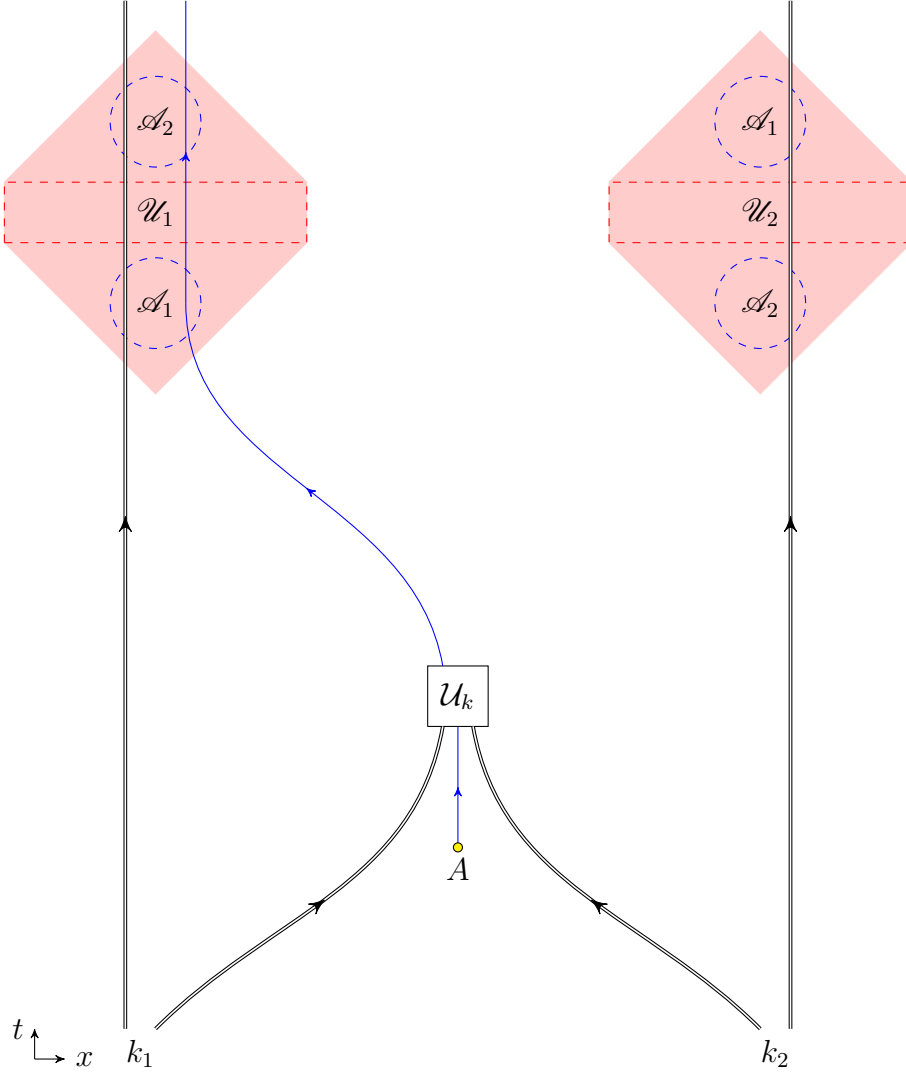
Figure 9: An example of a localize-exclude task and illustration of the protocol provided by theorem 8 for its completion. Near the start point the system A is encoded using the quantum one-time pad and sent (along the blue curve) through both authorized regions. The string k satisfies k = k_1 \oplus k_2 , so that k_1, k_2 form the two shares of a ((2, 2)) secret sharing scheme. k_1 is sent through \mathcal{A}_1 and \mathcal{A}_2 while avoiding \mathcal{U}_1 , while k_2 is sent through \mathcal{A}_1 and \mathcal{A}_2 while avoiding \mathcal{U}_2 . Consequently, each \mathcal{A}_i contains all of the classical shares k_i along with the encoded A system, while each \mathcal{U}_i is missing one k_i .
