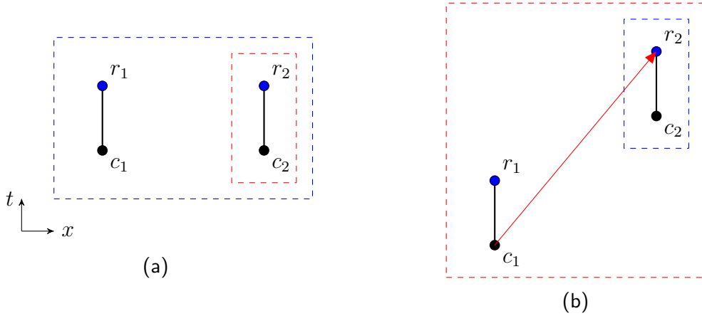
Figure 12: Illustration of condition (iii) in theorem 13. Dashed red boxes enclose unauthorized sets while dashed blue boxes enclose authorized sets. The condition states that every pairing (\mathcal{A}_a, \mathcal{U}_i) of authorized with unauthorized set must have either (a) \mathcal{A}_a \setminus \mathcal{U}_i \neq \emptyset or (b) \mathcal{U}_i \setminus \mathcal{A}_a is causally connected to \mathcal{A}_a .
