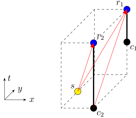
Figure 15: A summoning task on two diamonds in 2 + 1 dimensions. In this task r_1 is in the future light cone of c_2 , but r_2 is not in the future of c_1 . (In all figures, red arrows indicate causal curves.) Additionally, r_1 and r_2 are in the future light cone of s . To complete this summoning task, Alice pre-shares entanglement between s and c_1 . At s , Alice teleports the A system using the shared entanglement and then sends the classical teleportation data to both r_1 and r_2 . At c_1 , Alice routes the entangled particle she holds to r_1 if she receives b_1 = 1 , and routes the particle to r_2 otherwise. This example is due to Kent [10].
