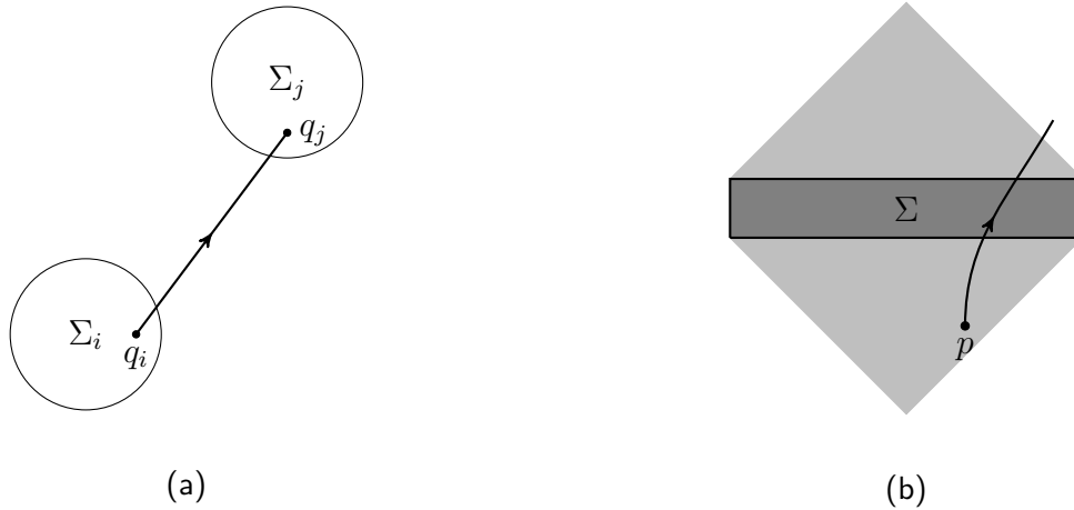
Figure 2: Two geometric notions used in the text. a) Two causally connected regions. Two spacetime regions \Sigma_i and \Sigma_j are said to be causally connected if there is a point q_i in \Sigma_i and q_j in \Sigma_j such that there is a causal curve from q_i to q_j , or from q_j to q_i . b) The domain of dependence (light grey) of a spacetime region \Sigma (dark grey). The domain of dependence is defined as the set of all points p in the spacetime such that all causal curves passing through p must also enter \Sigma .
