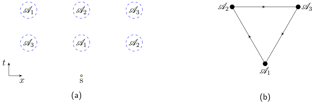
Figure 4: An example of a task with three authorized regions \mathcal{A}_1 , \mathcal{A}_2 and \mathcal{A}_3 . (a) The arrangement of the regions in spacetime, notice that each region consists of two disconnected ball-shaped regions. (b) The corresponding graph of causal connections, used in the proof of theorem 6 to construct the error-correcting code needed to complete the task.
