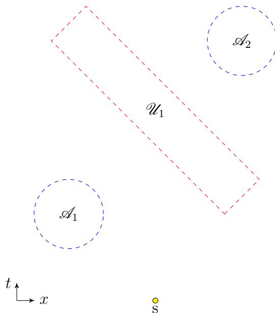
Figure 1: An example of a localize-exclude task. A single copy of an unknown quantum system is initially localized near the spacetime point s , and needs to be localized to within regions \mathcal{A}_1 and \mathcal{A}_2 , while avoiding region \mathcal{U}_1 . Theorem 8 shows that this is possible to do.
