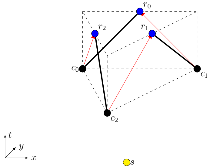
Figure 16: The three diamond task described in text. The known protocol for completing this task makes use of quantum error-correction: The system is encoded into a ((2, 3)) secret sharing scheme with one share sent to each of the call points c_i . The shares are then routed to r_{i+1 \bmod 3} if b_i = 0 , and to r_i if b_i = 1 . This task is the simplest example of a summoning task which Alice can complete if there is a guarantee Bob will make only one call, but not if Bob may make an arbitrary number of calls.
