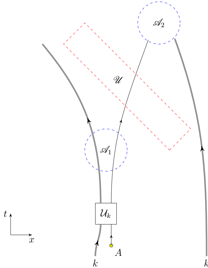
Figure 7: Illustration of the protocol for completing a localize-exclude task with two authorized regions and one unauthorized region that satisfy the conditions of theorem 8. In the distant past, Alice prepares copies of the classical string k . She brings one copy of k to each of \mathcal{A}_1 and \mathcal{A}_2 along a path which does not cross \mathcal{U} — this is always possible by condition (iii). She must also bring the classical string to the start point s , and encode the A system using the quantum one-time pad [22]. The overall state on A and its purifying system R is then of the form (\mathcal{U}_k \otimes \mathcal{I})|\Psi\rangle_{AR} . The encoded system A is sent through both authorized regions. By following this protocol both authorized regions contain k and the encoded A system, while the unauthorized region contains the encoded system only.
