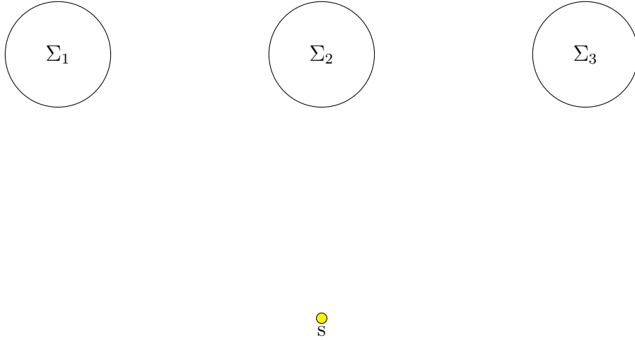
Figure 10: Example of the embedding of a secret sharing scheme with arbitrary access structure into a localize-exclude task. We consider a secret sharing scheme that involves three parties, and has authorized sets S_1 = \{1, 2\} , S_2 = \{2, 3\} and S_3 = \{1, 2, 3\} , with all other subsets of parties deemed unauthorized. In the corresponding localize-exclude task, the three parties become three causally disjoint spacetime regions \Sigma_1, \Sigma_2 and \Sigma_3 . Further, this localize-exclude task has authorized regions \mathcal{A}_1 = \Sigma_1 \cup \Sigma_2 , \mathcal{A}_2 = \Sigma_2 \cup \Sigma_3 and \mathcal{A}_3 = \Sigma_1 \cup \Sigma_2 \cup \Sigma_3 . The start point s has been placed at an early enough time that all the \Sigma_i are in its future light cone.
