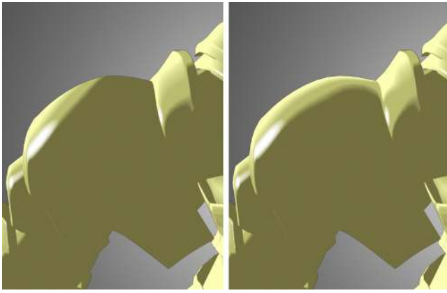
Figure 7: Modifying shading with gradations. Here our prototype system has been used to make a directional lighting setup appear to be a more dramatic back-lit situation.
