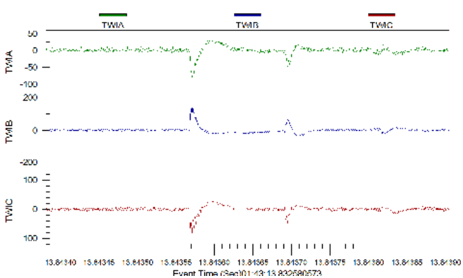
Fig. 32. Phase currents at Goshen for a BG fault at 98.98 km from the Goshen terminal.
