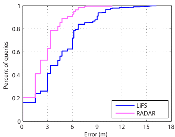
Figure 20: CDF of localization error.
