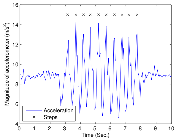
Figure 7: The acceleration pattern for 10 steps.
