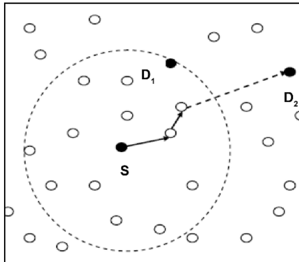
Figure 16. Route Setup in IHLAR [64].
