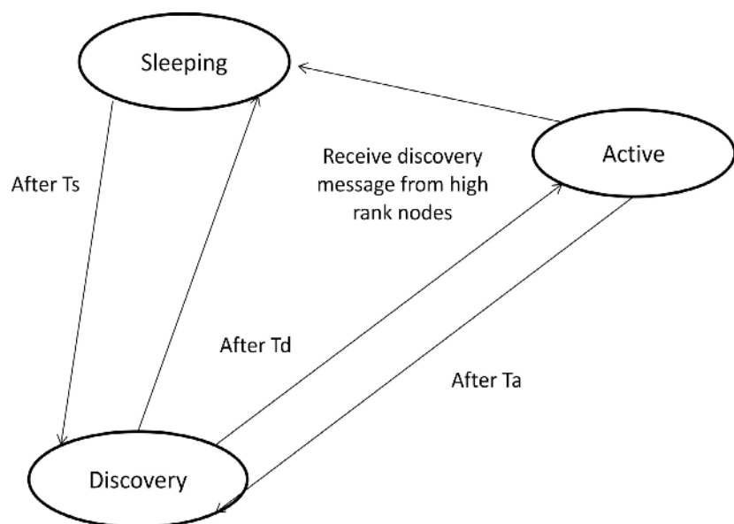
Figure 11. State transitions in GAF [59].
