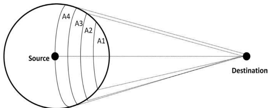
Figure 20. Priority region in GeRaF: increasing priority from A4 to A1 [70].
