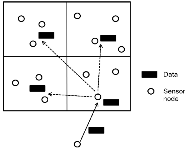
Figure 12. Recursive geographic forwarding in GEAR [60].
