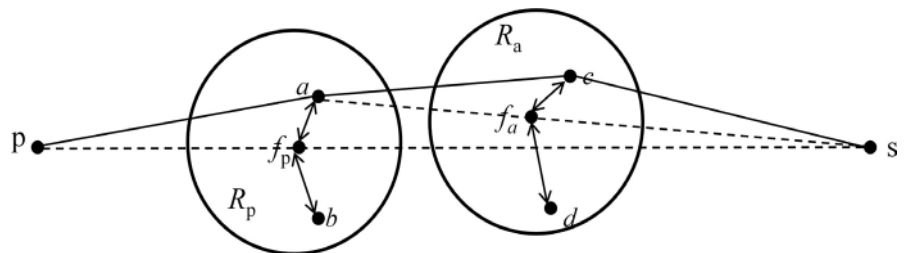
Figure 22. Forwarding process of EEGR [78].
