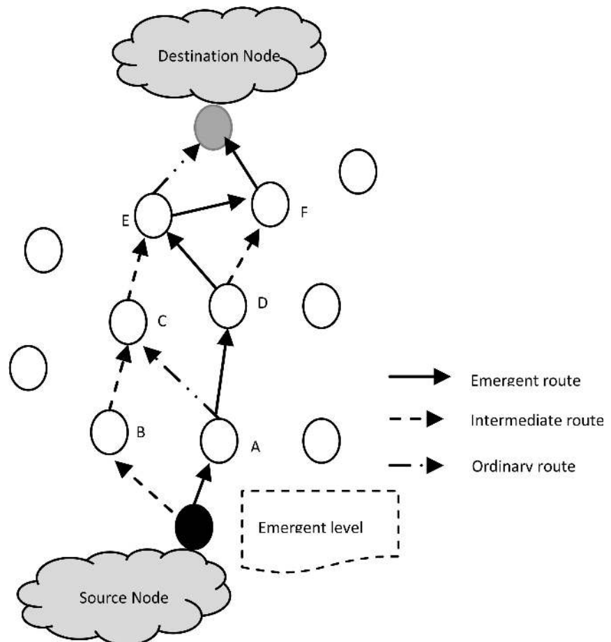
Figure 30. A routing path of LARP from source to destination [94].
