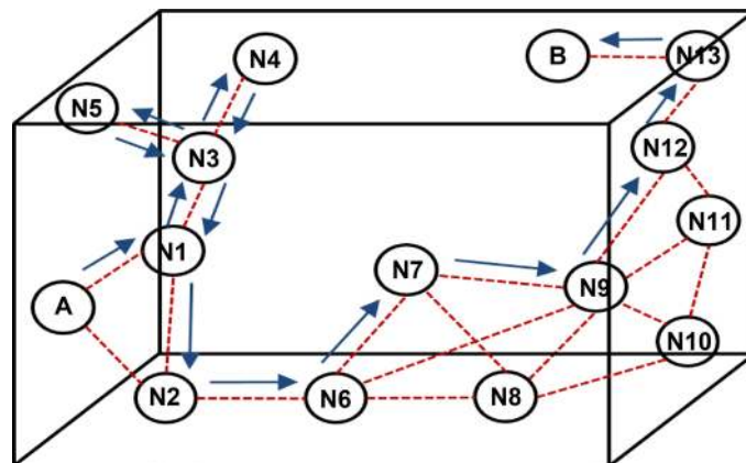
Figure 17. Example of LBRP routing a packet from node A to node B [65].
