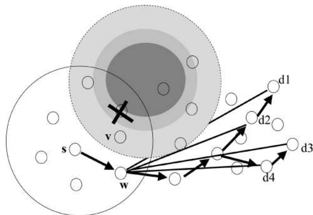
Figure 31. Selecting the best energy path and forwarding packets in LMR; s: source, d1 ~ d4: destination, v, w: neighbour nodes [95].
