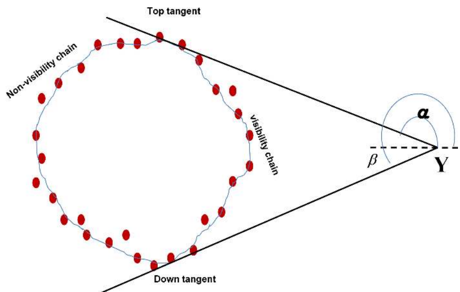
Figure 26. Visibility chain of a given node y consists of the nodes which are located between the two tangents and the destination.
