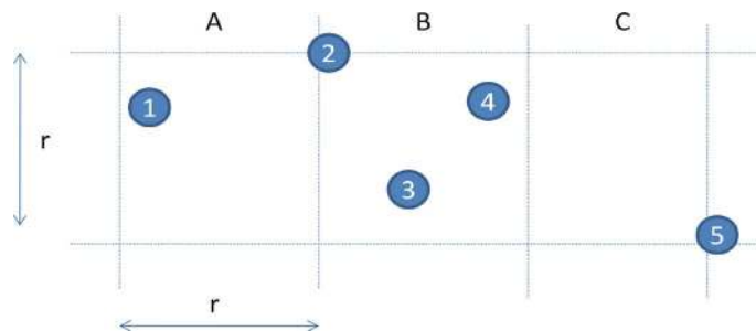
Figure 10. A simple example of virtual grid in GAF [59].
