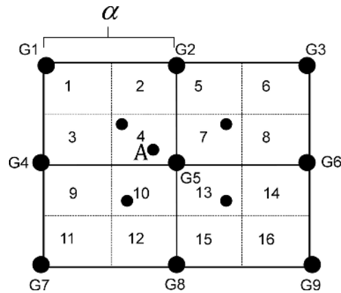
Figure 21. The grid node selection process [73].
