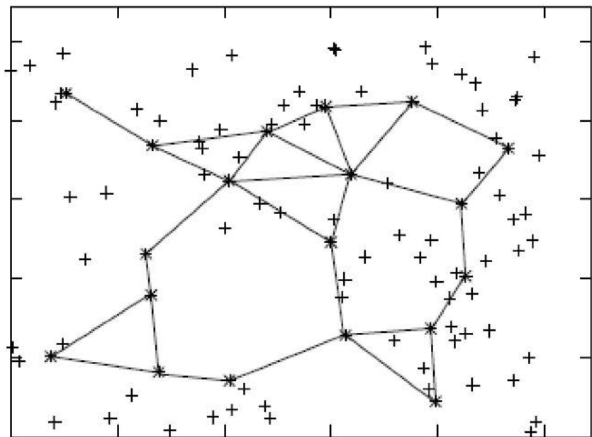
Figure 28. An example of routing path in SPAN [91].
