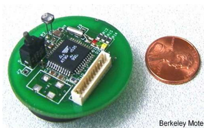
Figure 3. Berkeley mote [17].
