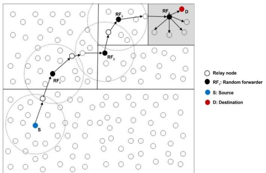
Figure 14. Routing among zones in ALERT [62].
