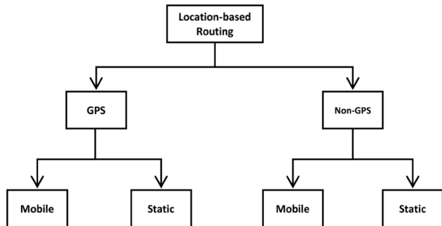
Figure 5. Categorization of location-based routing protocols.
