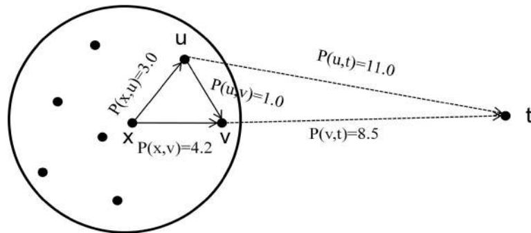
Figure 15. A node x selects its neighbour node to reach destination [63].
