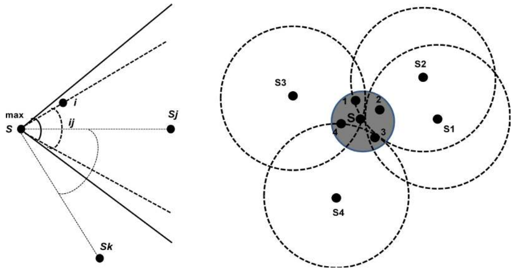
Figure 23. D_s = \{S1, S2, S3\} , D1 = \{S2, S3\} , D2 = \{S2, S1\} , D3 = \{S1\} , D4 = \{S3\} . The maximum allowed apex angle, \alpha_{max} , and the apex of the shrink-est cone in the S_j direction that contain i, ai, j , are depicted [82].
