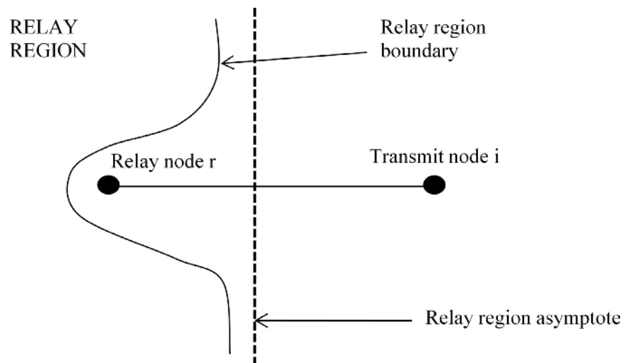
Figure 7. Relay region of the transmit-relay node pair in MECN [57].
