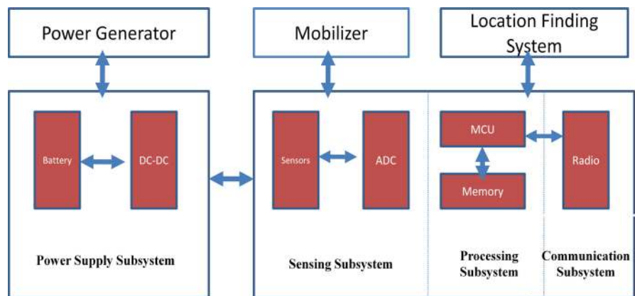
Figure 2. Architecture of a typical sensor node.
