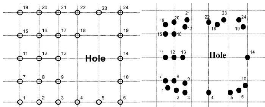
Figure 24. Example shows the node and 1st-level virtual position of node in the network [84].
