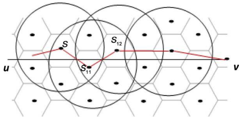
Figure 19. A routing path of BVGF [69].
